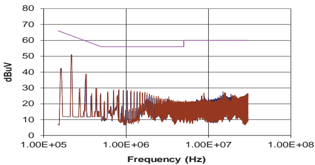
NMV0505TSAC (Quasi-Peak)
