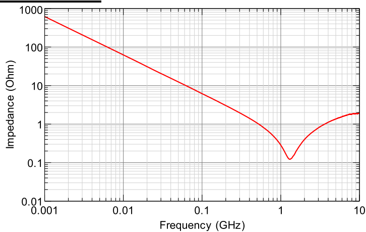
Figure 2 - 270pF WLSC measurement results (Impedance characteristic versus Frequency in shunt mode)
