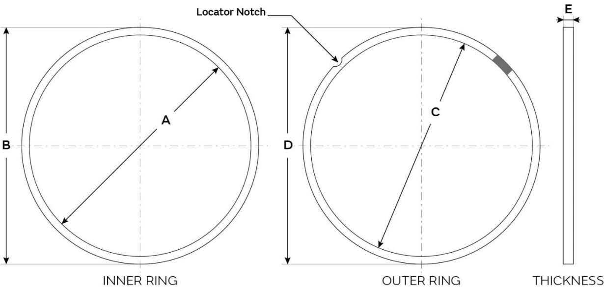
Figure 12 – Grip Ring drawing
