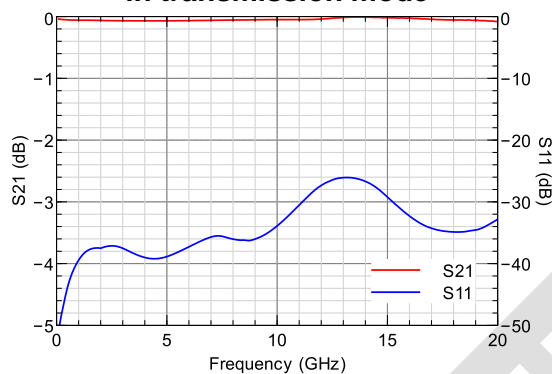
Figure 2 - 47nF ULSC Measured results (module of S-parameters)
