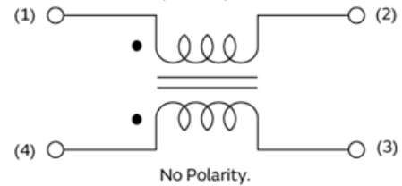
Equivalent circuit (Note1)
