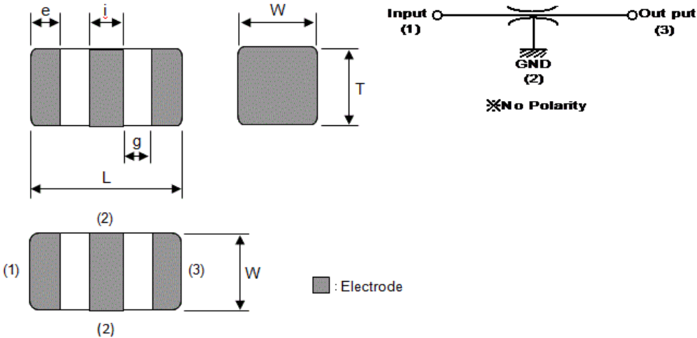
image:Dimension
