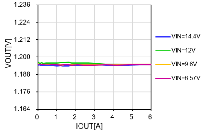
Figure 18. V_{OUT} vs. Load Current and Line Voltage
