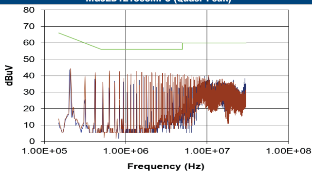
MGJ2D121505MPC (Quasi-Peak)
