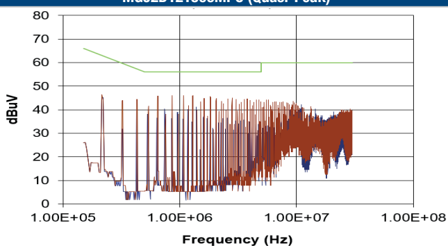
MGJ2D121509MPC (Quasi-Peak)
