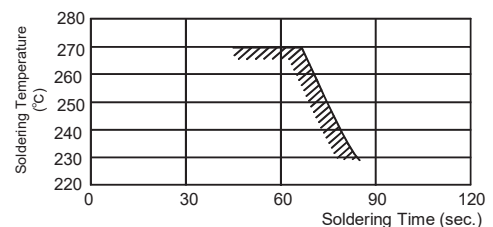
[Allowable Reflow Soldering Temperature and Time]
