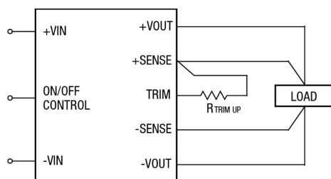
Figure 9. Trim Connections to Increase Output Voltage
