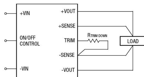
Figure 10. Trim Connections to Decrease Output Voltage
