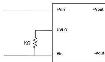
Figure 3. Under Voltage Lockout Configuration
