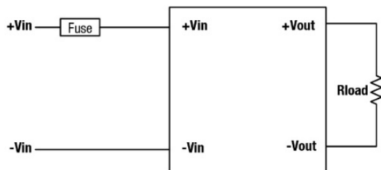
Figure 2. Input Fusing
