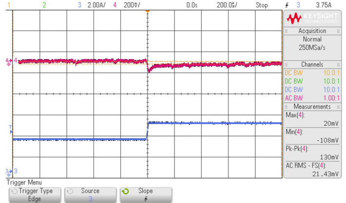
Output Ripple@20MHz BW, V_{in} = 72Vdc , Full Load with 2200uF output capacitance
