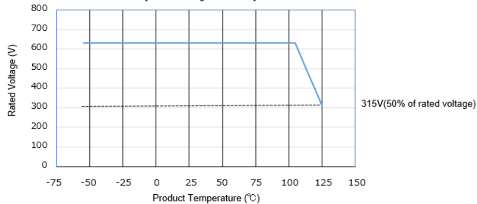
Fig:Derating
