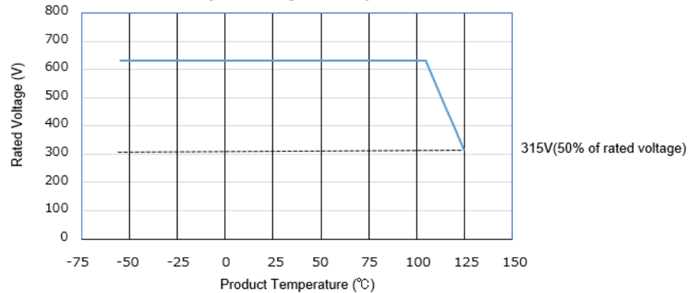
Fig:Derating
