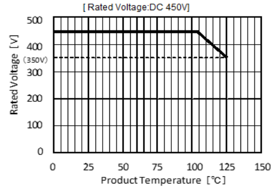
Fig:Derating
