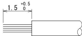
3 Fig.1 Recommended cable preparation dimensions
