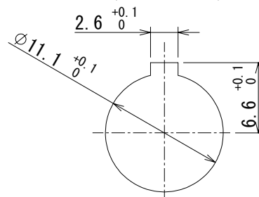
Panel cutout (t=0.7 to 2)
