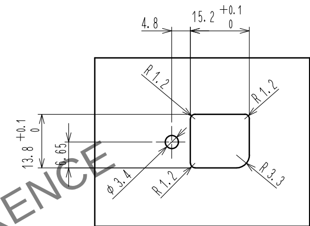
RECOMMENDED PANEL CUT-OUT FOR GT5-1PP-HU(70) (1:1)
