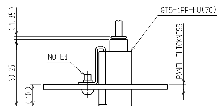
MATED CONNECTORS FOR GT5-1PP-HU(70) (1:1)
