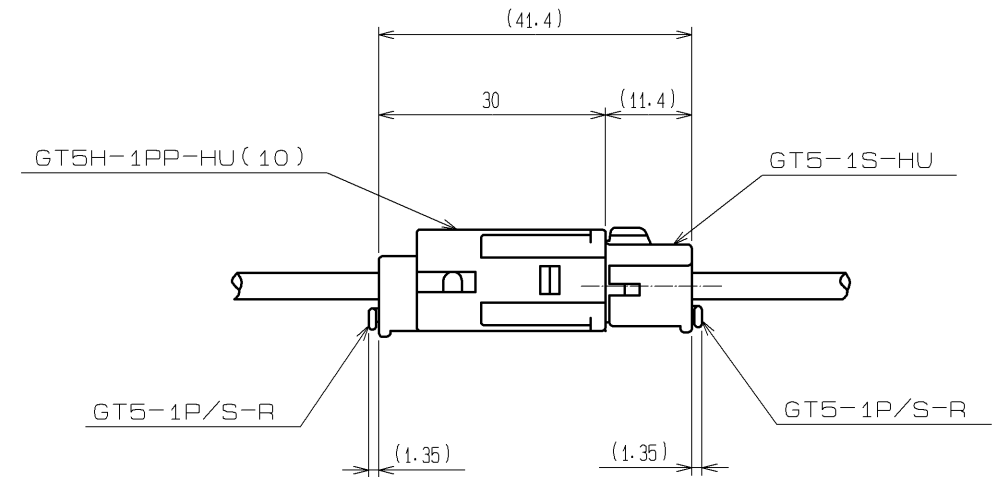
MATED CONNECTORS
