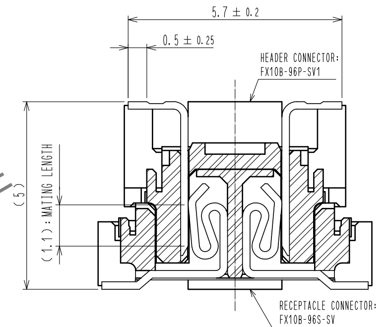
CROSS CUT SECTION (10:1)
