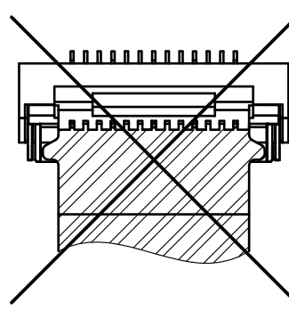
When FPC TAB is on right and left guides for positioning FPC, it causes the loose connection.
