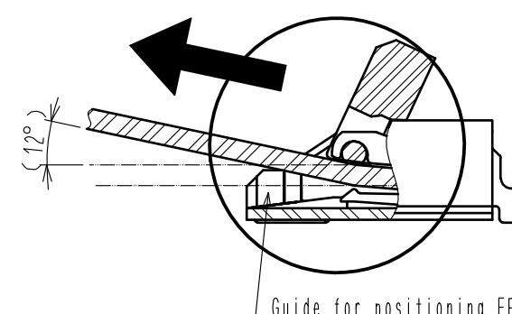
Guide for positioning FPC
