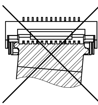
When FPC TAB is on right or left guide for positioning FPC, it causes the loose connection.
