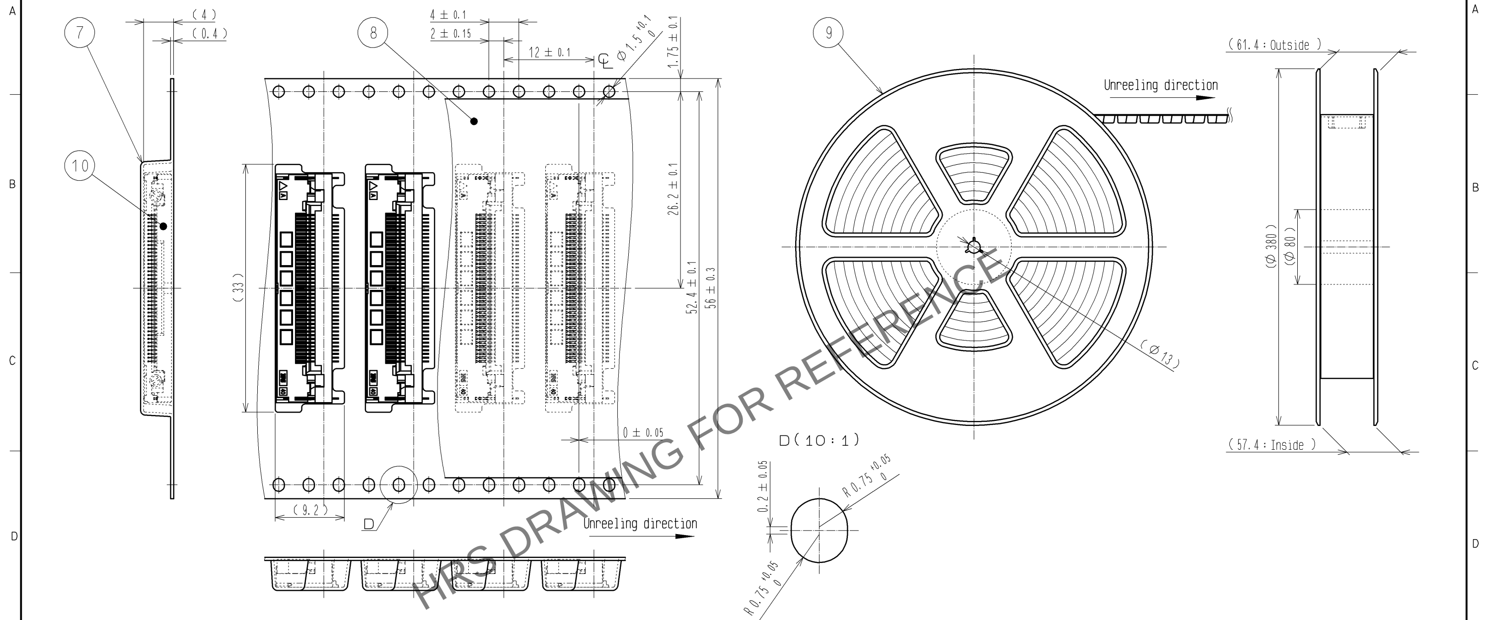
Embossed carrier tape dimensions (2:1)
