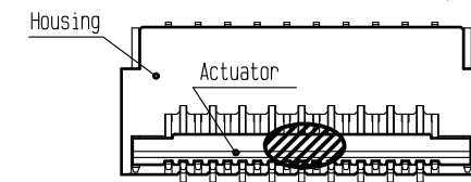
[Actuator operation area (lock and release)] (Top view)
