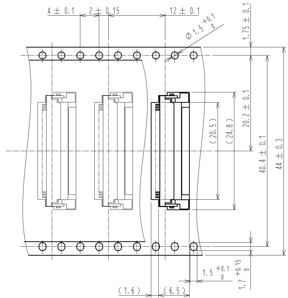
EMBOSSED CARRIER TAPE DIMENSION(2:1)
