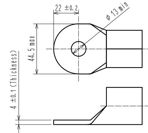
Figure.2 Applicable Contact (Commercial item)(Free)
