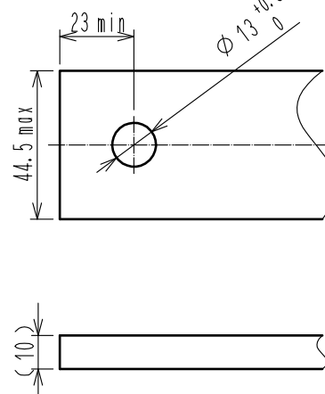
Figure.3 Recommended bus bar dimensions.
