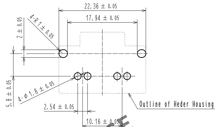
Recommended PCB Layout (Board thickness: t=1.6 \pm 0.1 mm)
