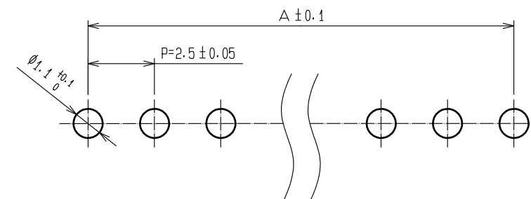
RECOMMENDED PATTERN(5:1)
