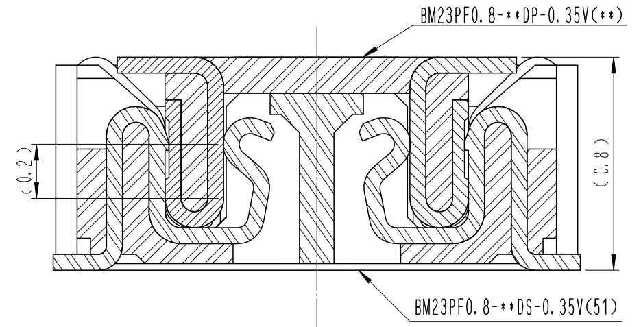
ENGAGEMENT FIGURE (50:1)
