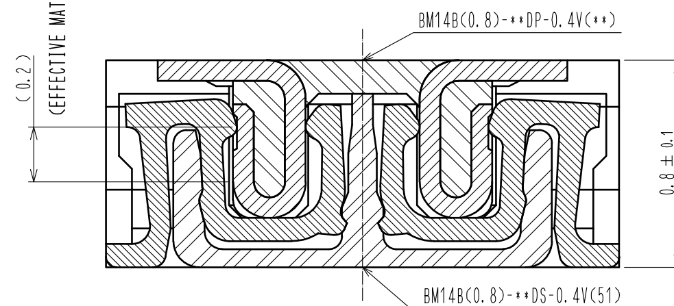
ENGAGEMENT FIGURE (50:1)
