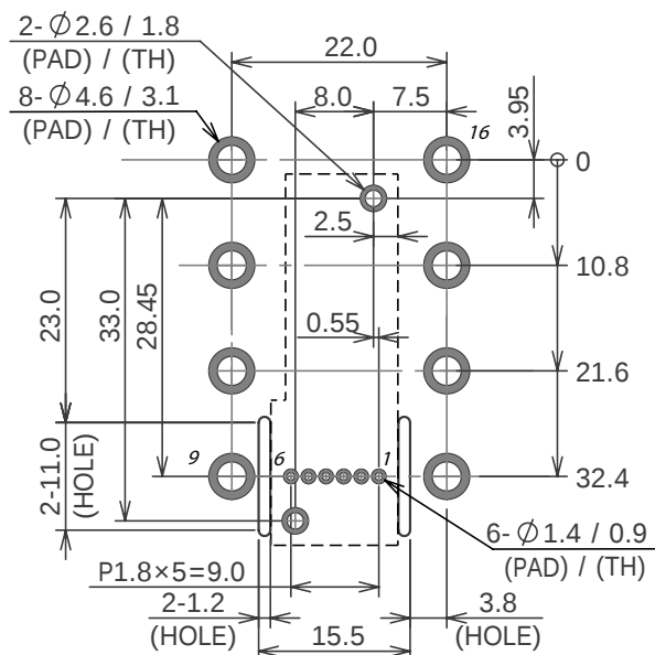
Component side
