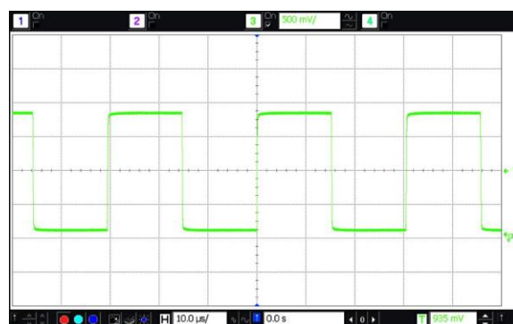
Figure 14. LVCMOS Output Waveform ( V_{Swing} = 1.8 V, SiT1533AI-H4-DCC-32.768)
