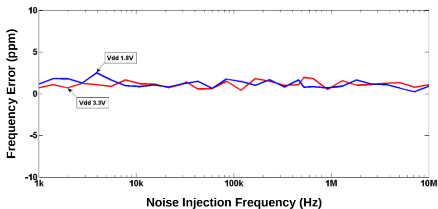
Figure 12. Power Supply Noise Rejection ( \pm 150 mV Noise)
