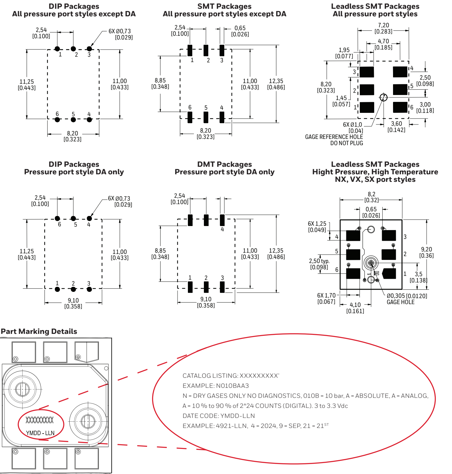
Figure 13. Recommended PCB Layout and Part Marking Details
