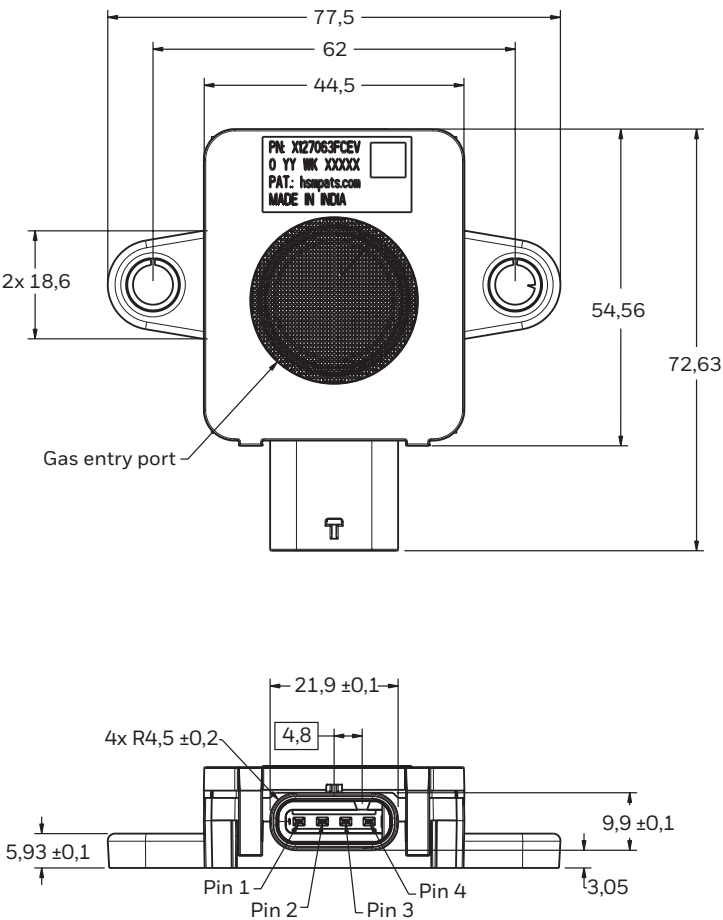
Figure 1. Product Dimensions (mm)
