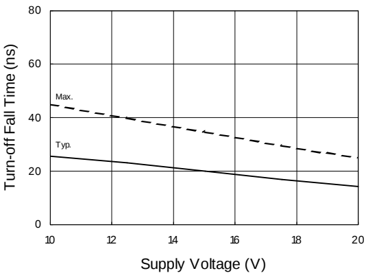
Figure 17B. Turn-Off Fall Time vs. Supply Voltage
