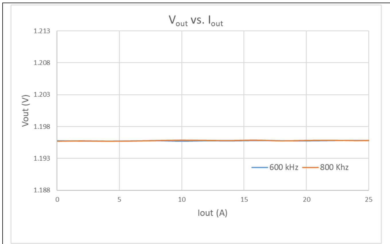
Figure 24 TDA38725 V OUT regulation (12 V IN , 1.2 V OUT , no airflow, 150 nH, 600/800 kHz, T a = 25°C)
