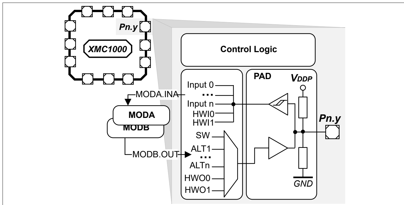
Figure 10 Simplified Port Structure
