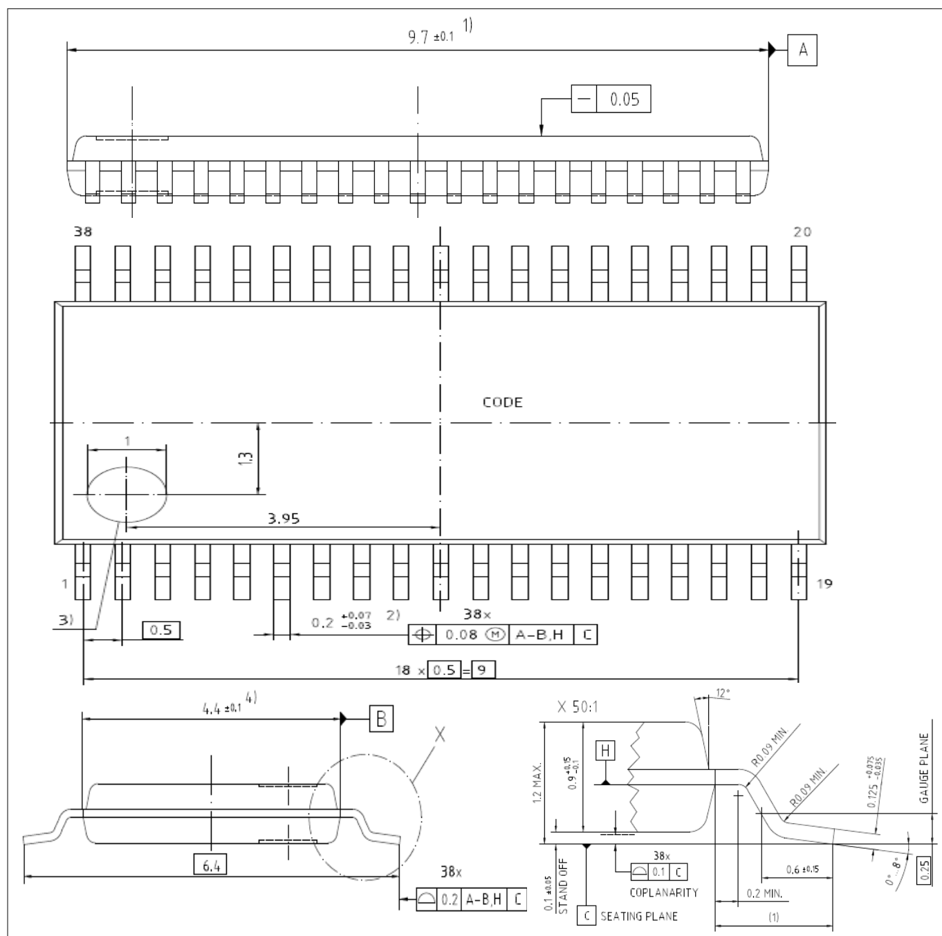
Figure 29 PG-TSSOP-38-9
