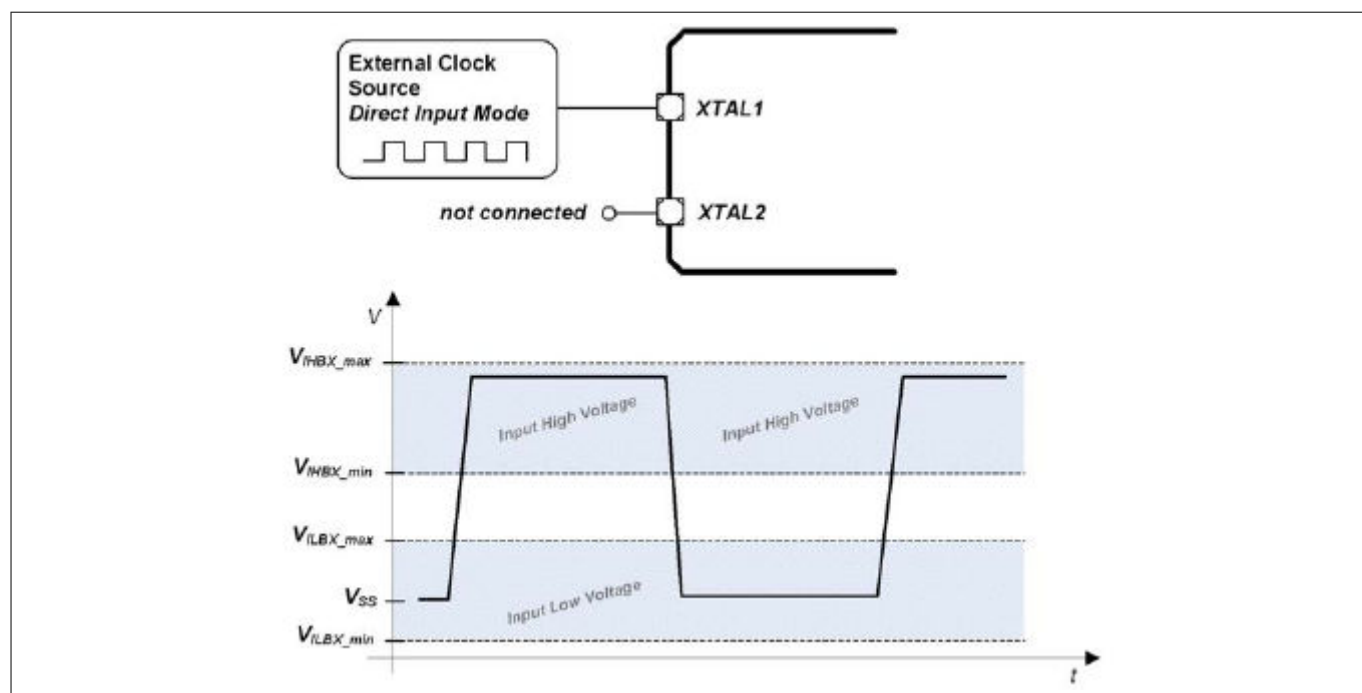
Figure 16 Oscillator in Direct Input Mode
