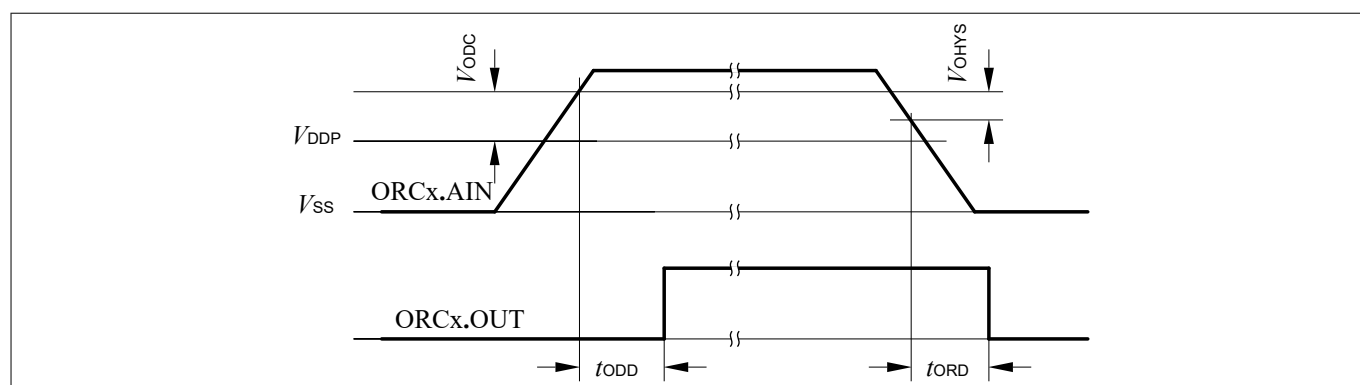
Figure 13 ORCx.OUT Trigger Generation
