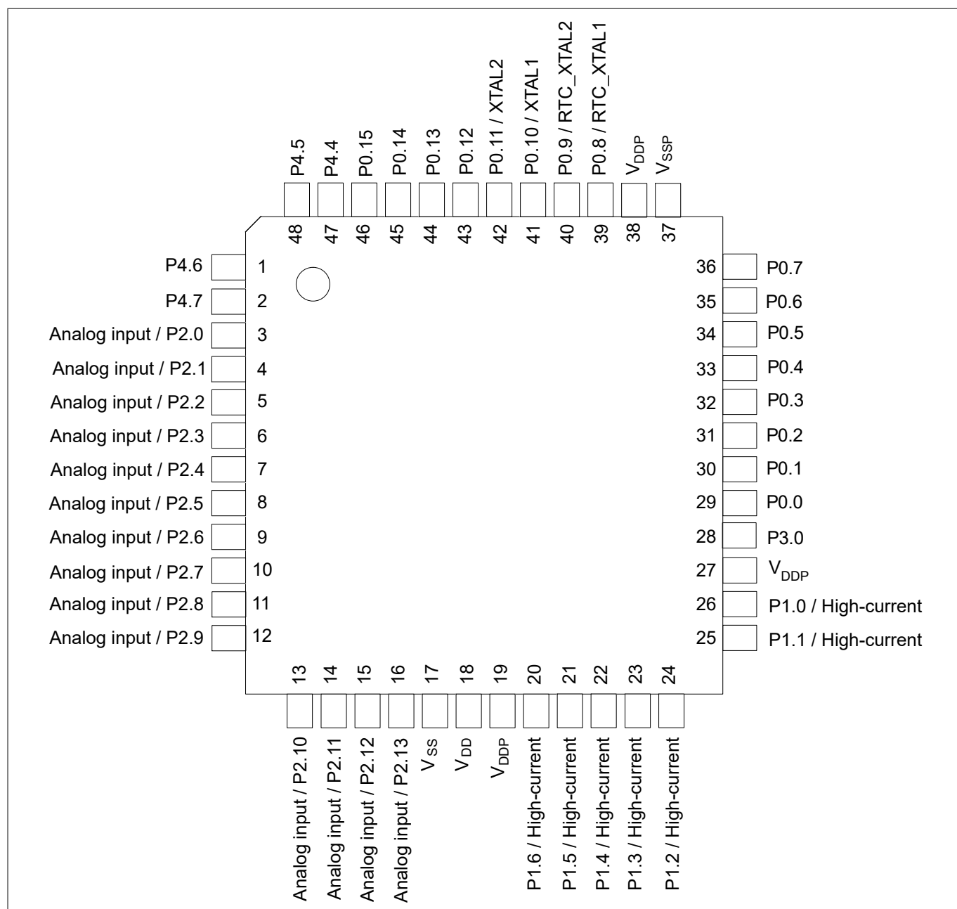
Figure 8 XMC1400 PG-VQFN-48-73 Pin Configuration (top view)
