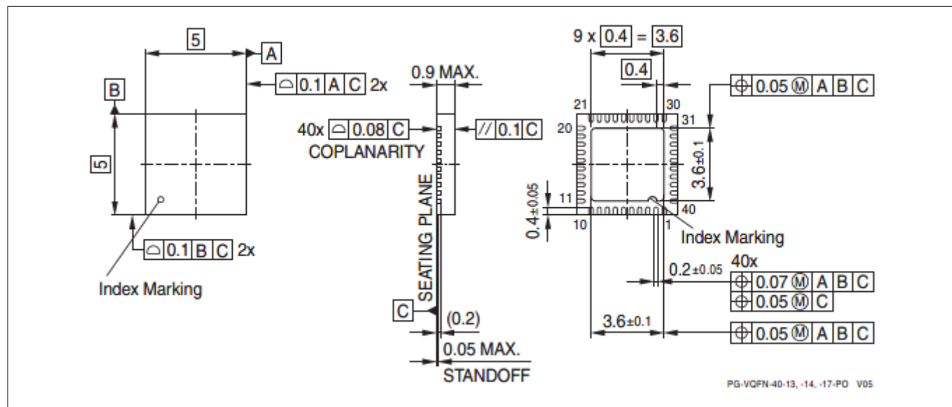
Figure 30 PG-VQFN-40-17
