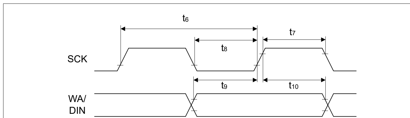
Figure 28 USIC IIS Slave Receiver Timing
