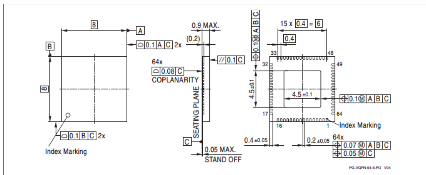
Figure 33 PG-VQFN-64-6
