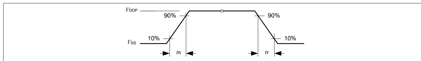
Figure 20 Rise/Fall Time Parameters
