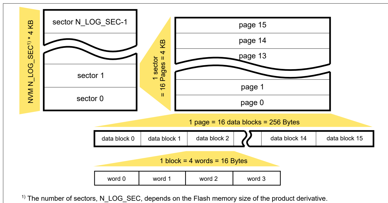
Figure 19 Logical Structure of the Flash
