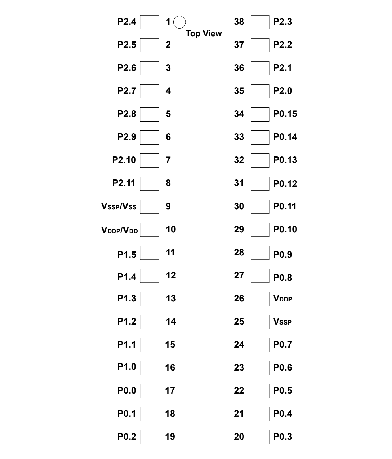
Figure 6 XMC1400 PG-TSSOP-38-9 Pin Configuration (top view)
