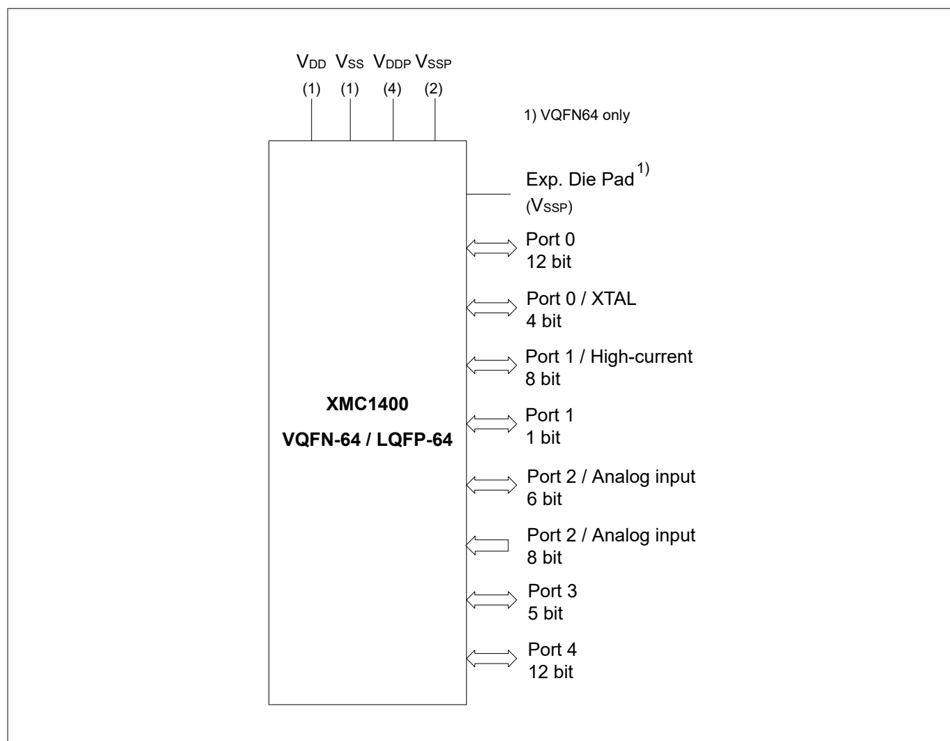
Figure 5 XMC1400 Logic Symbol for PG-LQFP-64-26/PG-VQFN-64-6
