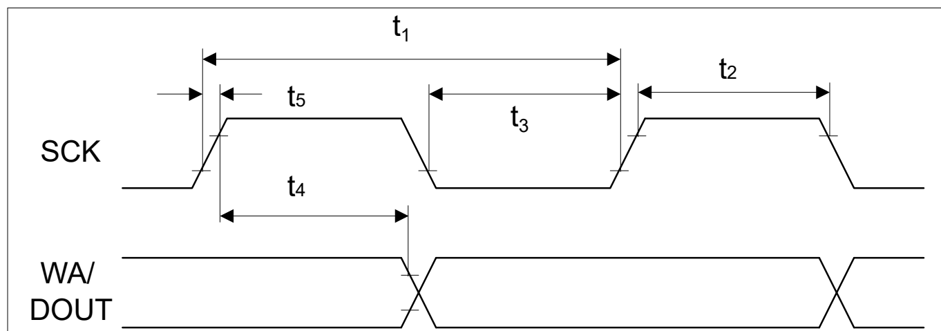
Figure 27 USIC IIS Master Transmitter Timing
