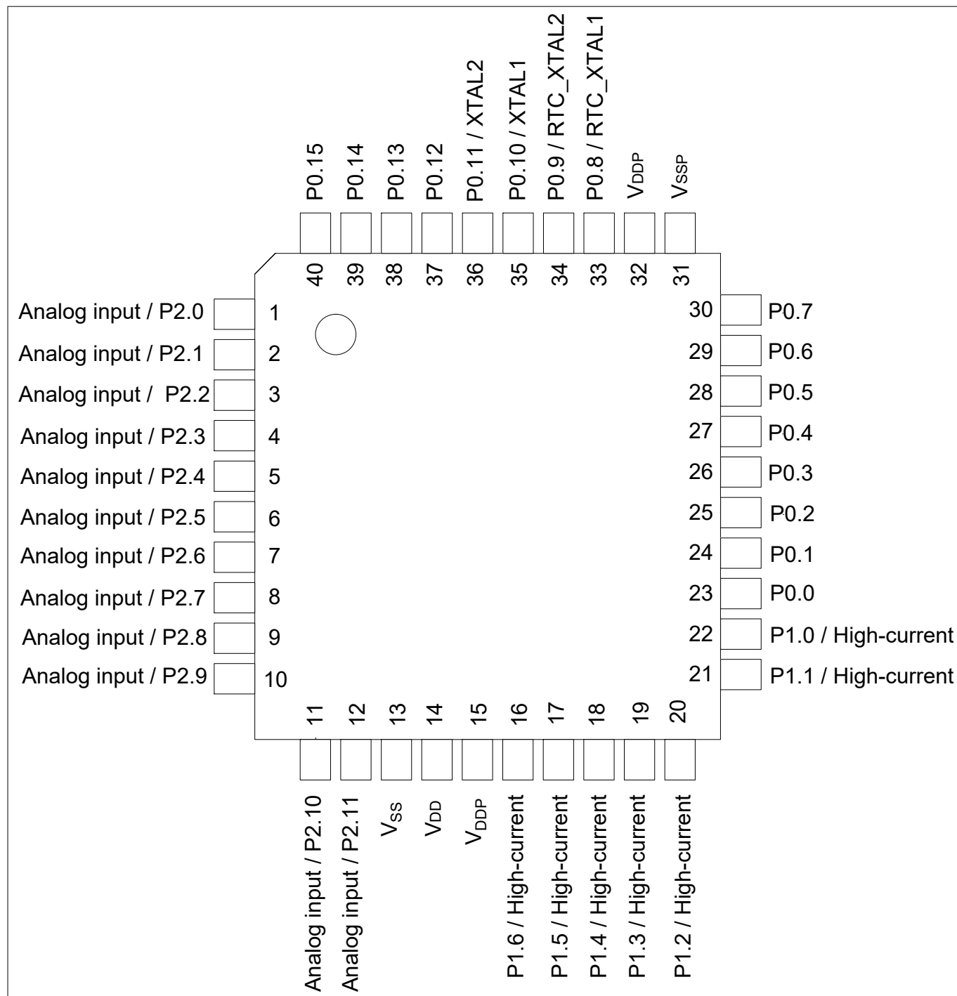
Figure 7 XMC1400 PG-VQFN-40-17 Pin Configuration (top view)
