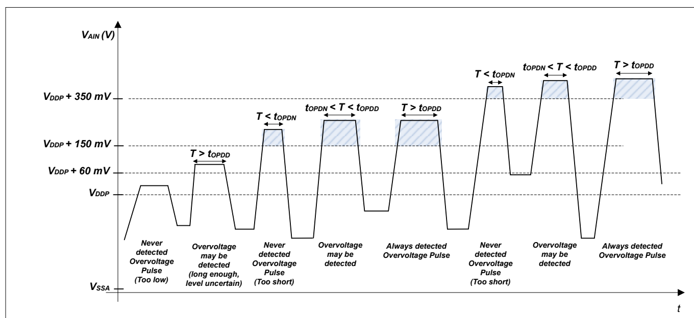
Figure 14 ORC Detection Ranges
