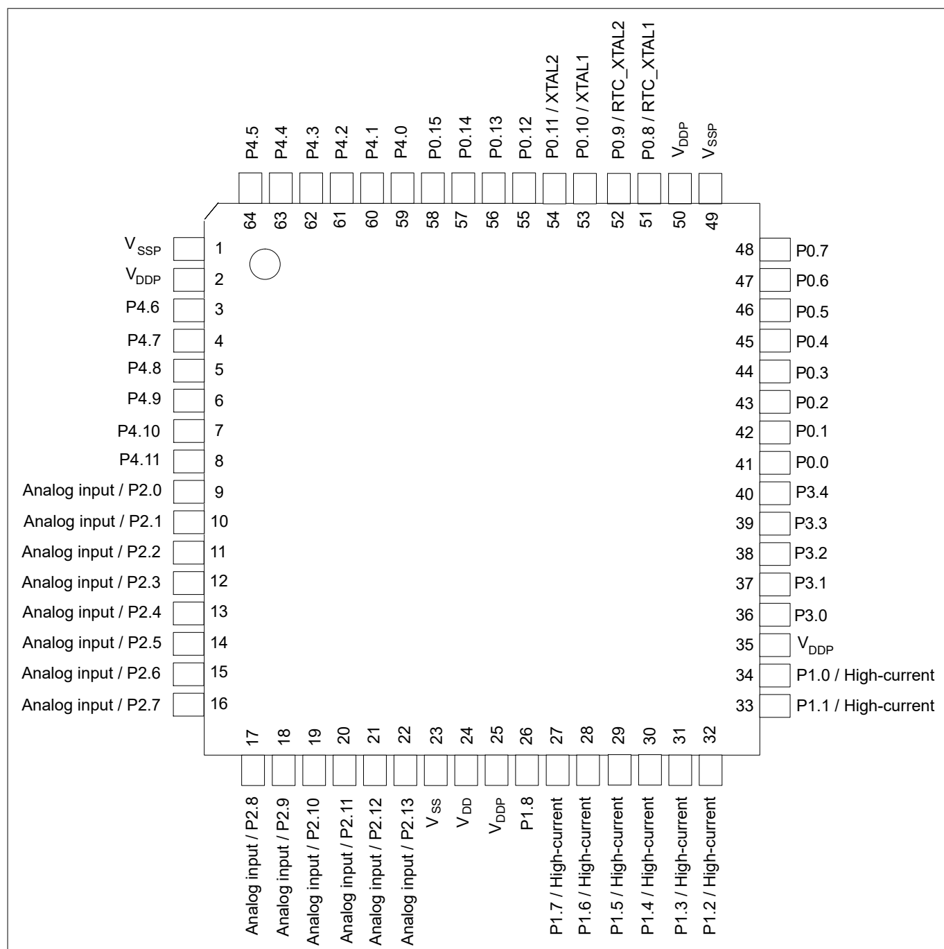
Figure 9 XMC1400 PG-LQFP-64-26/PG-VQFN-64-6 Pin Configuration (top view)
