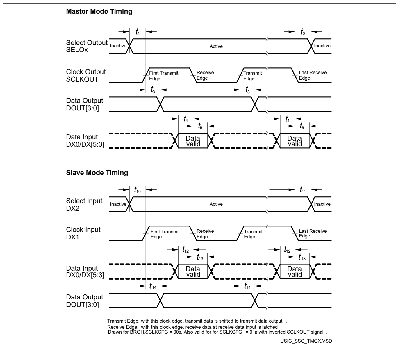
Figure 25 USIC - SSC Master/Slave Mode Timing
