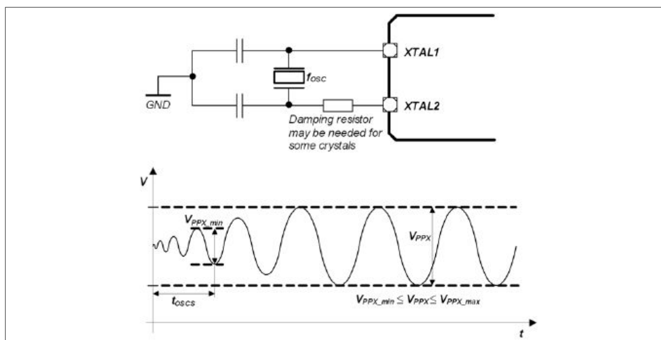
Figure 15 Oscillator in Crystal Mode
