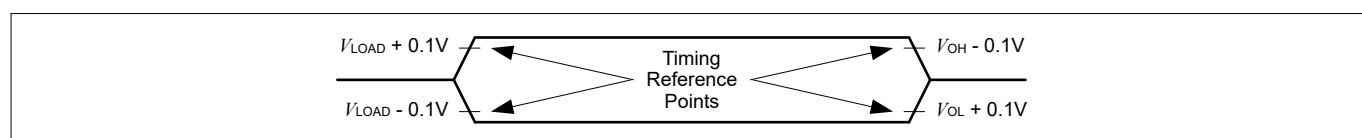
Figure 22 Testing Waveform, Output High Impedance
