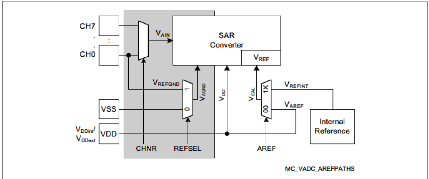
Figure 12 ADC Voltage Supply
