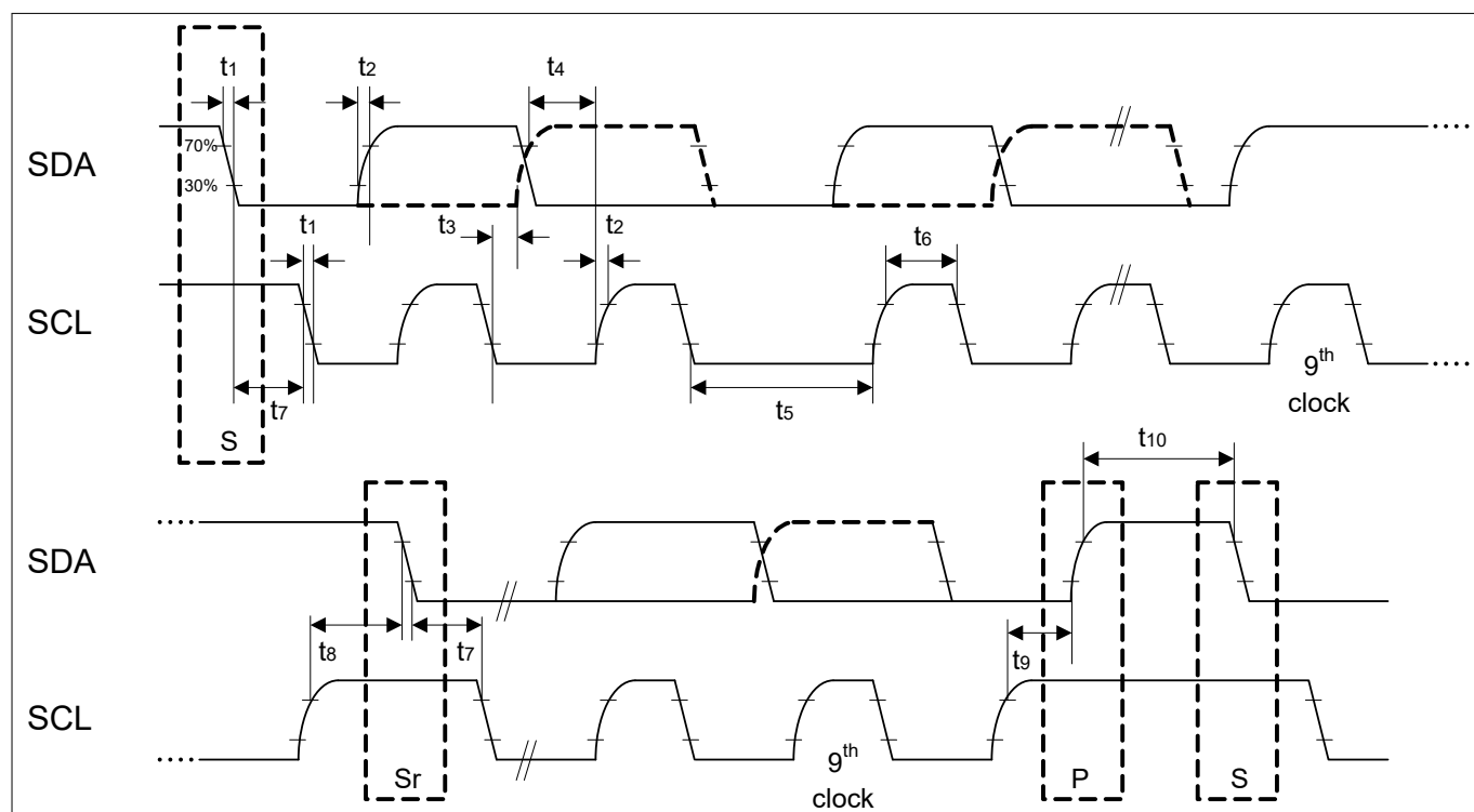
Figure 26 USIC IIC Timing
