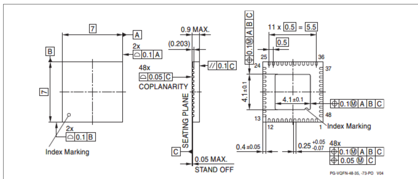
Figure 31 PG-VQFN-48-73
