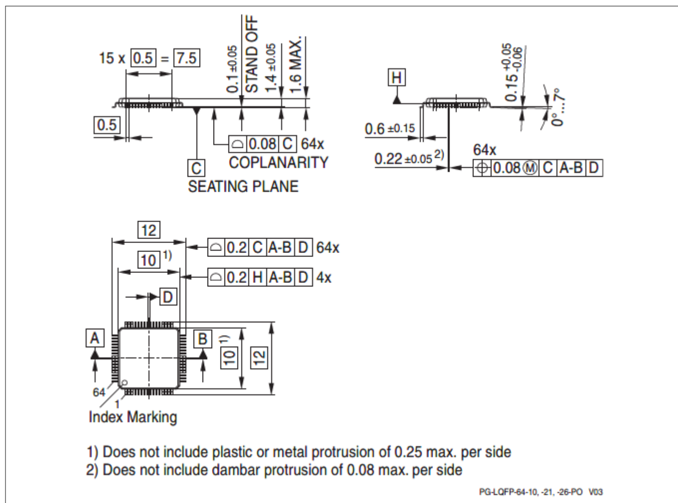
Figure 32 PG-LQFP-64-26
