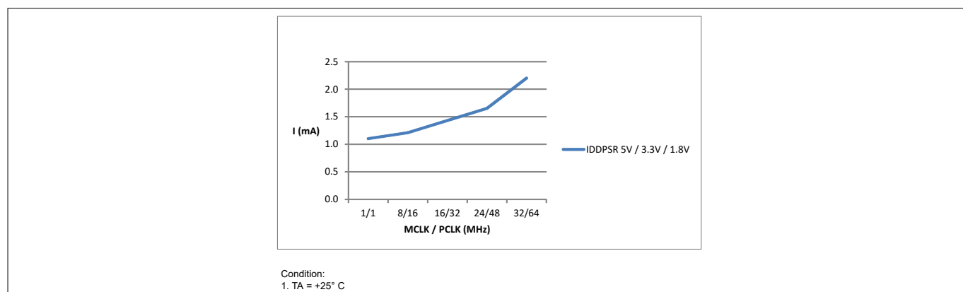
Figure 18 Sleep mode, peripherals clocks disabled, Flash powered down: Supply current I_{DDPSD} over supply voltage V_{DDP} for different clock frequencies
