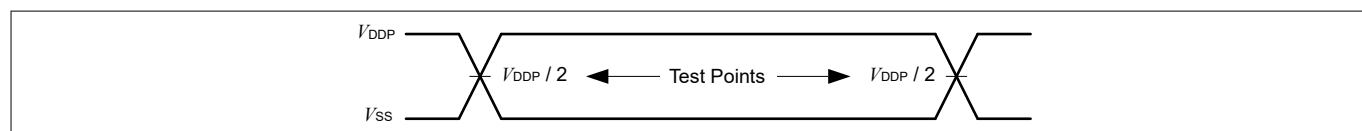
Figure 21 Testing Waveform, Output Delay
