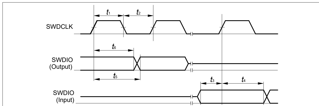
Figure 24 SWD Timing
