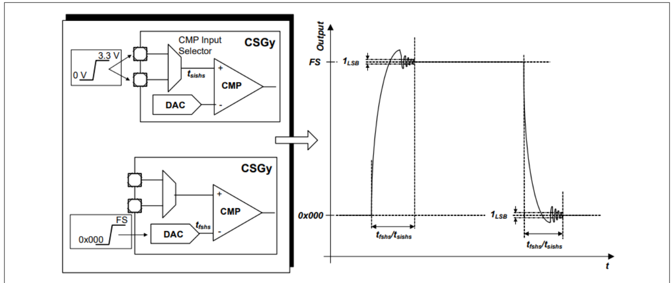
Figure 20 DAC and Input Selector Propagation Delay
