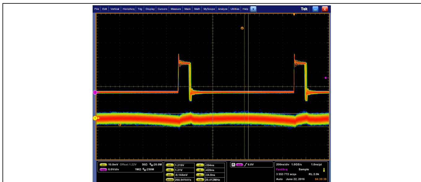
Figure 20 MIDDLE→SW_NODE, BOTTOM→RIPPLE
