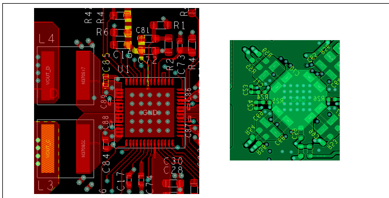
Figure 13 Layout details
