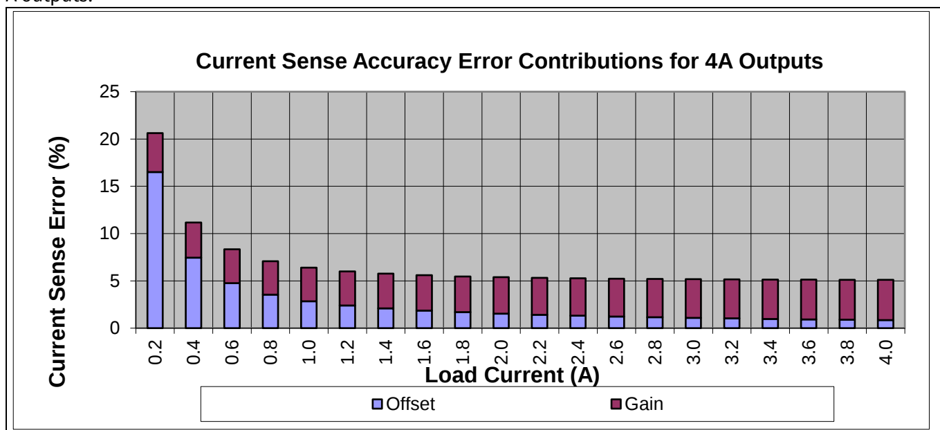
Figure 22 Current reporting
