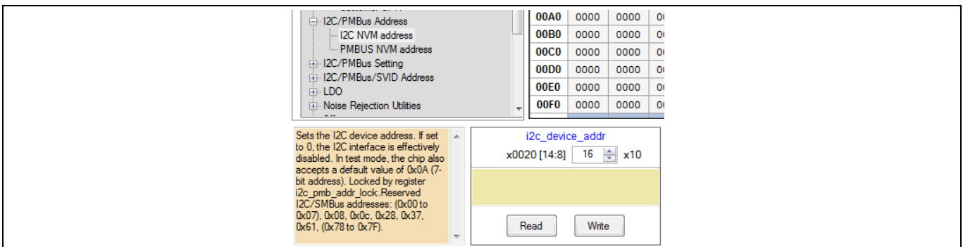
Figure 5 I2C address
