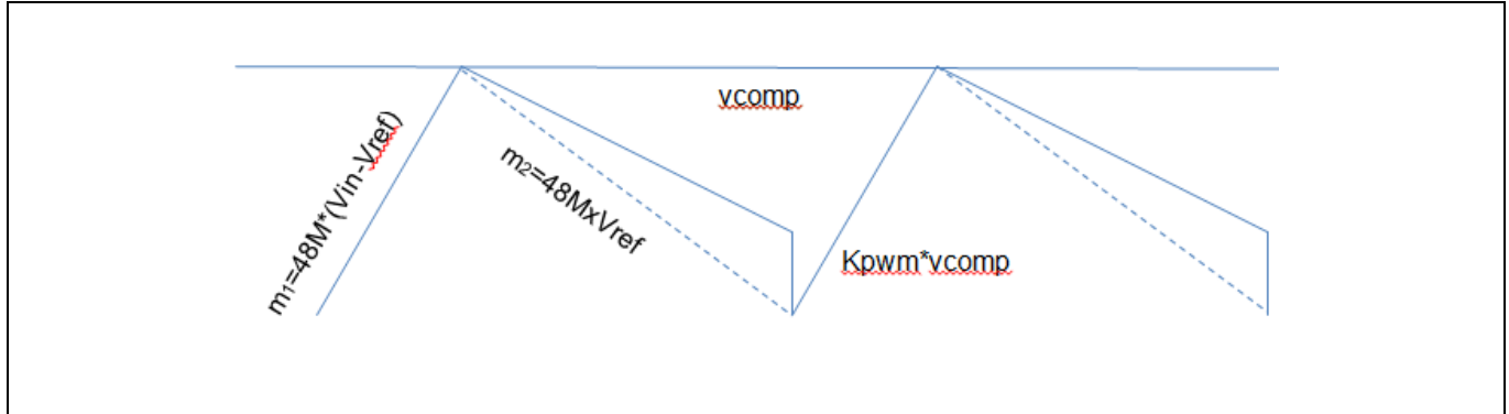
Figure 40 Vcomp
