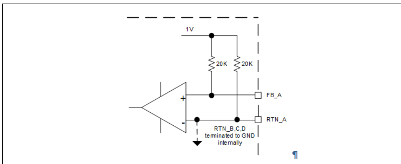
Figure 27 FB_x
