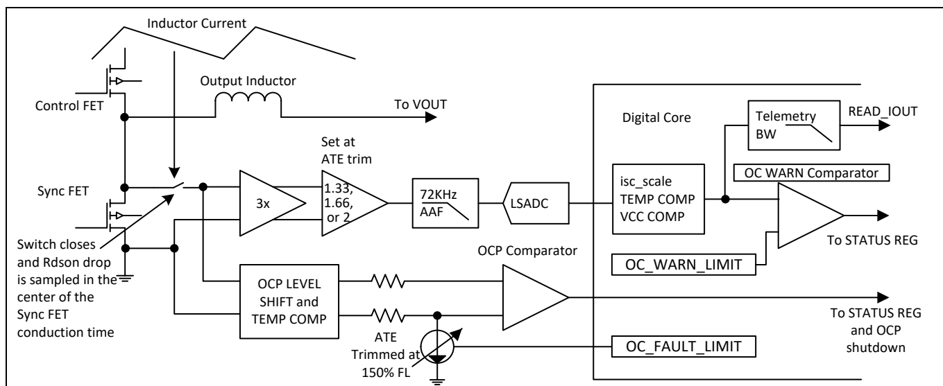
Figure 21 Current settings
