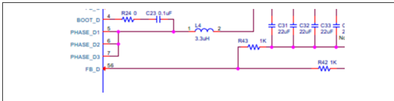
Figure 26 VOUT scaling
