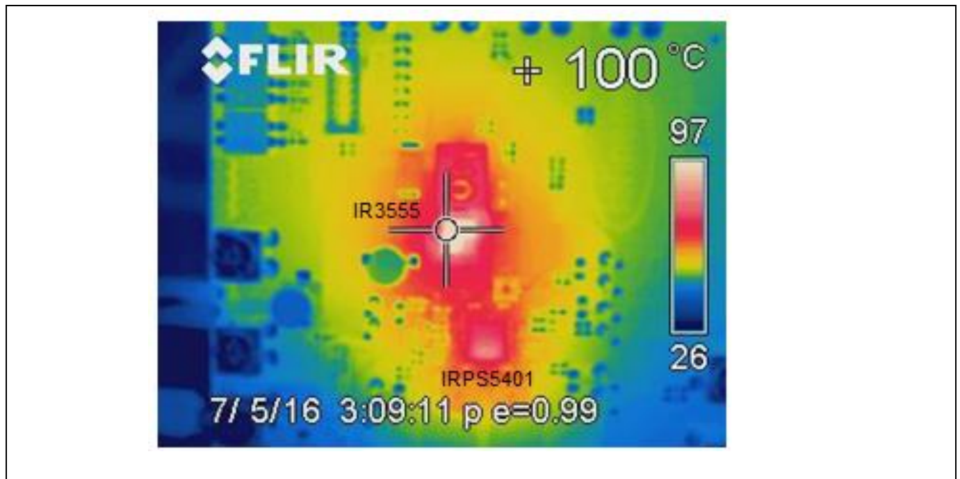
Figure 71 IR3555 thermal image
