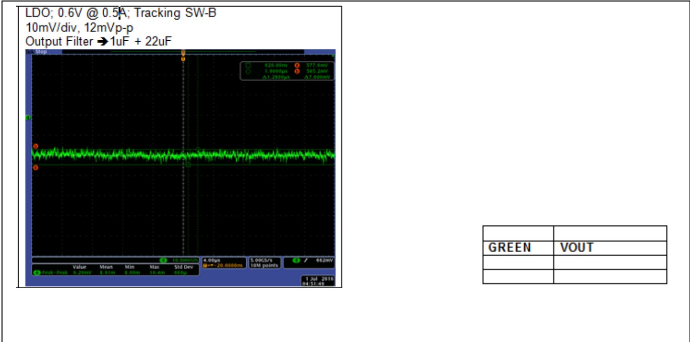
Figure 61 Output ripple
