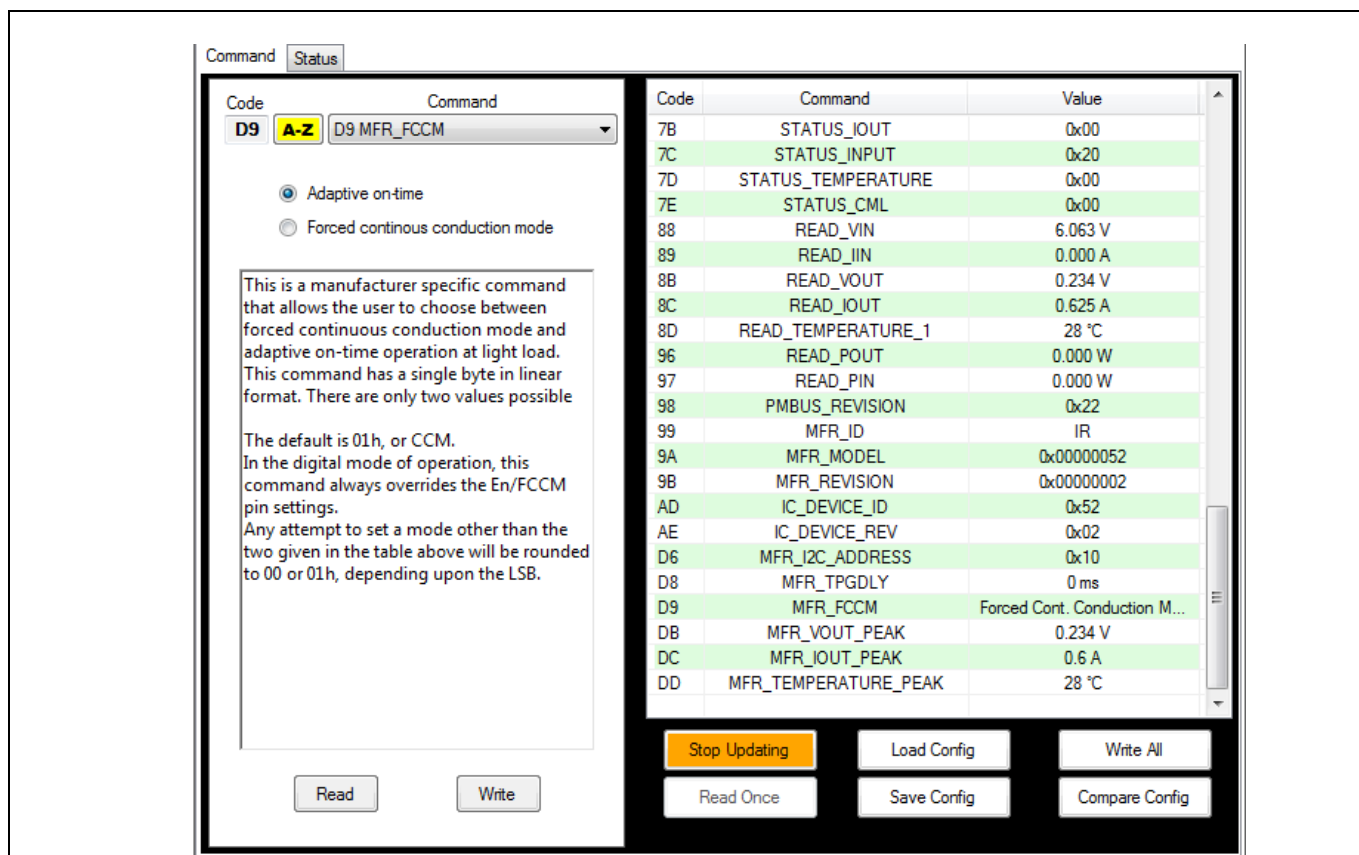
Figure 14 AOT mode
