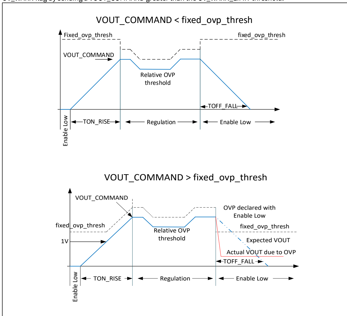
Figure 24 VOUT_COMMAND
