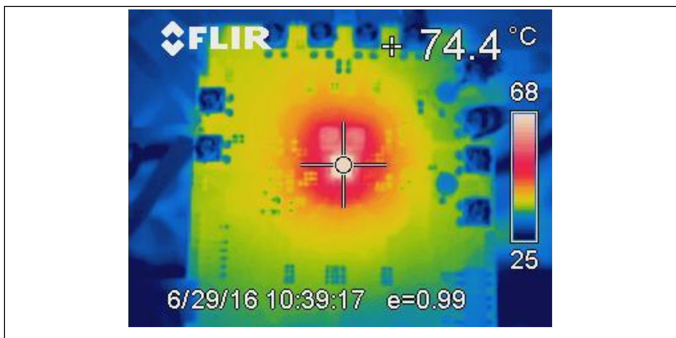
Figure 55 Thermal image of entire board
