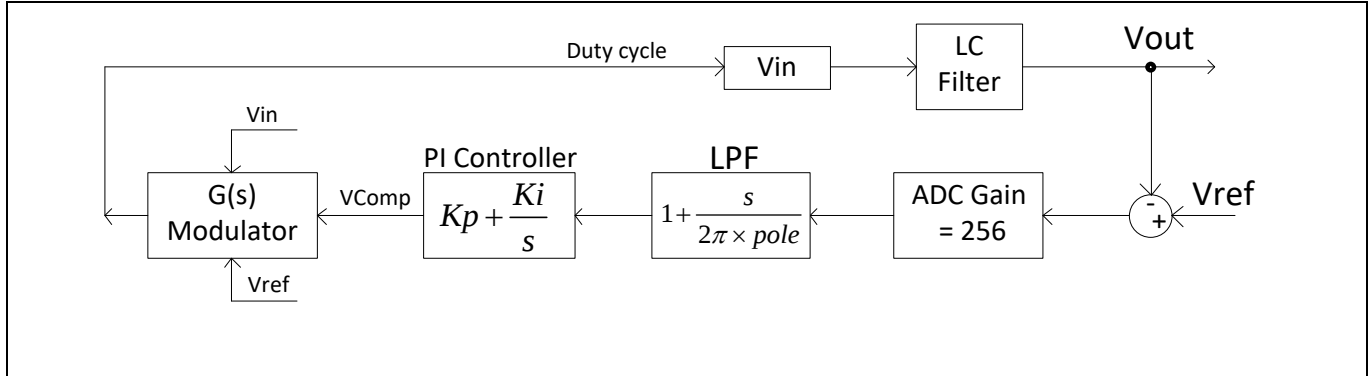
Figure 39 Emulator
