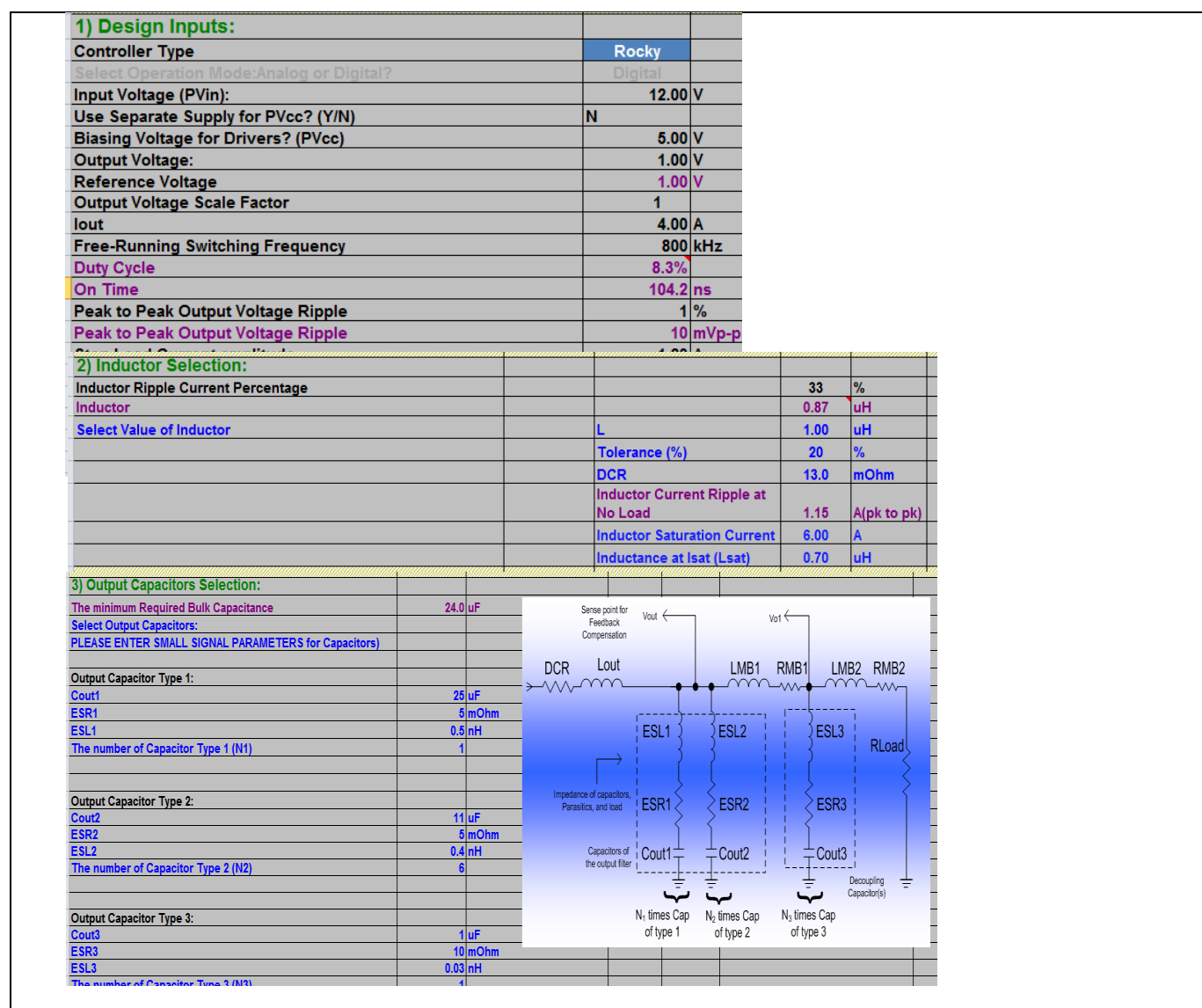
Figure 41 Design Tool
