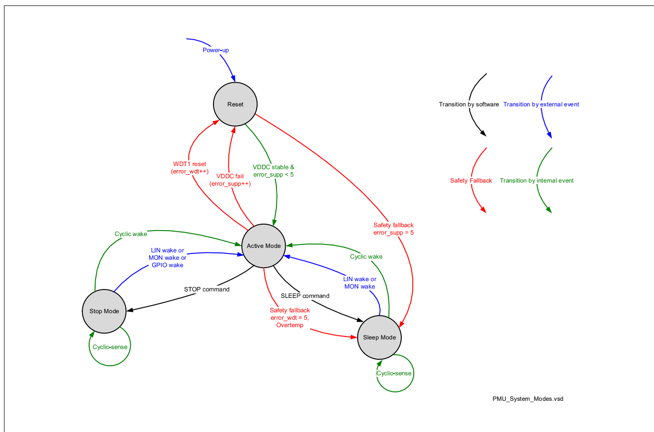
Figure 3 Power Control State Diagram
