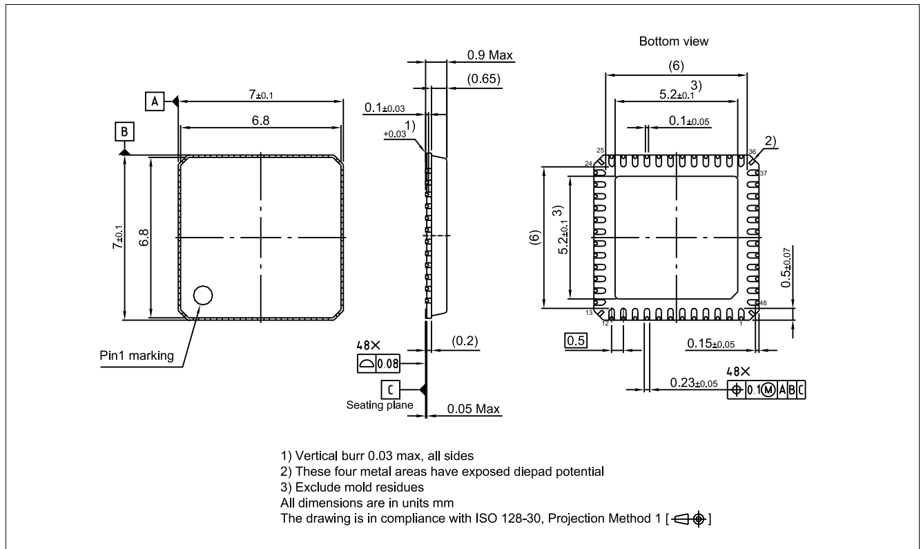
Figure 92 PG-VQFN-48-31
