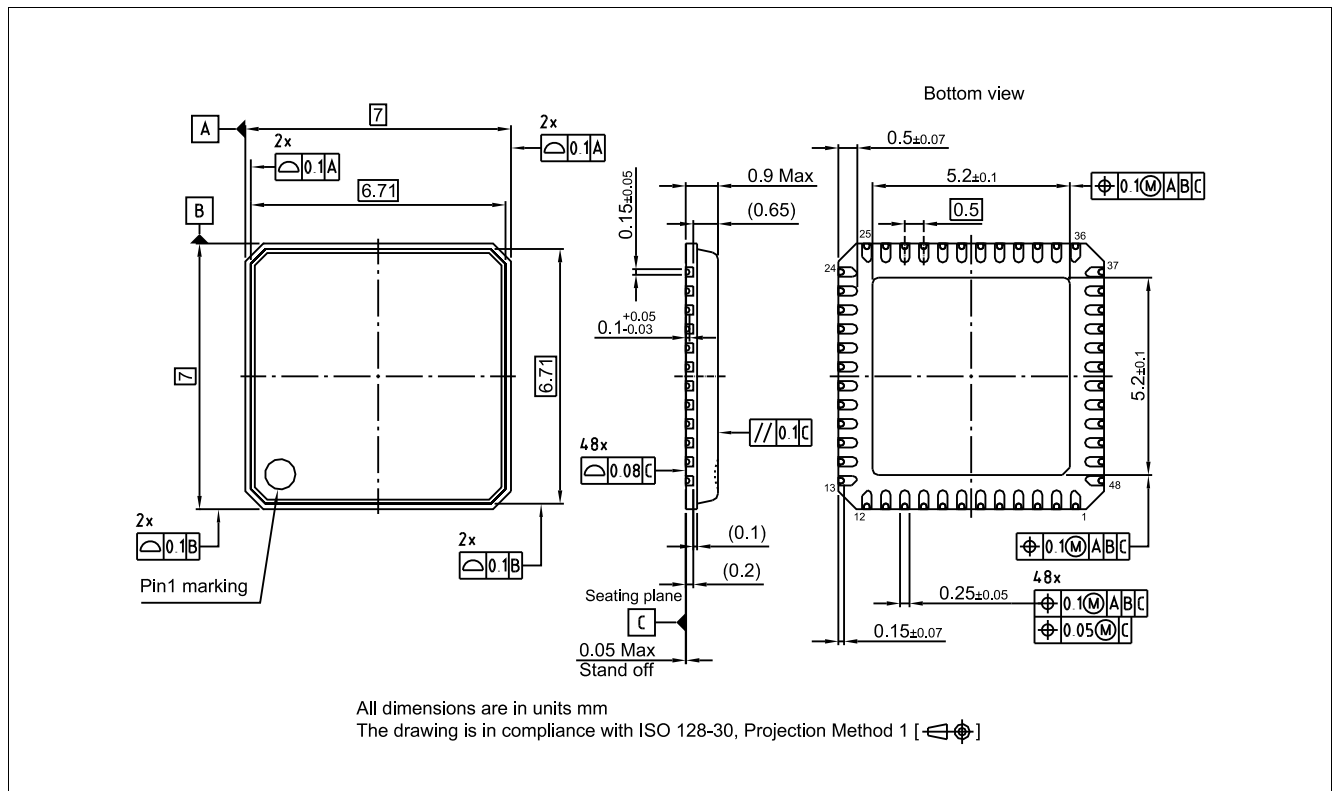
Figure 93 PG-VQFN-48-79
