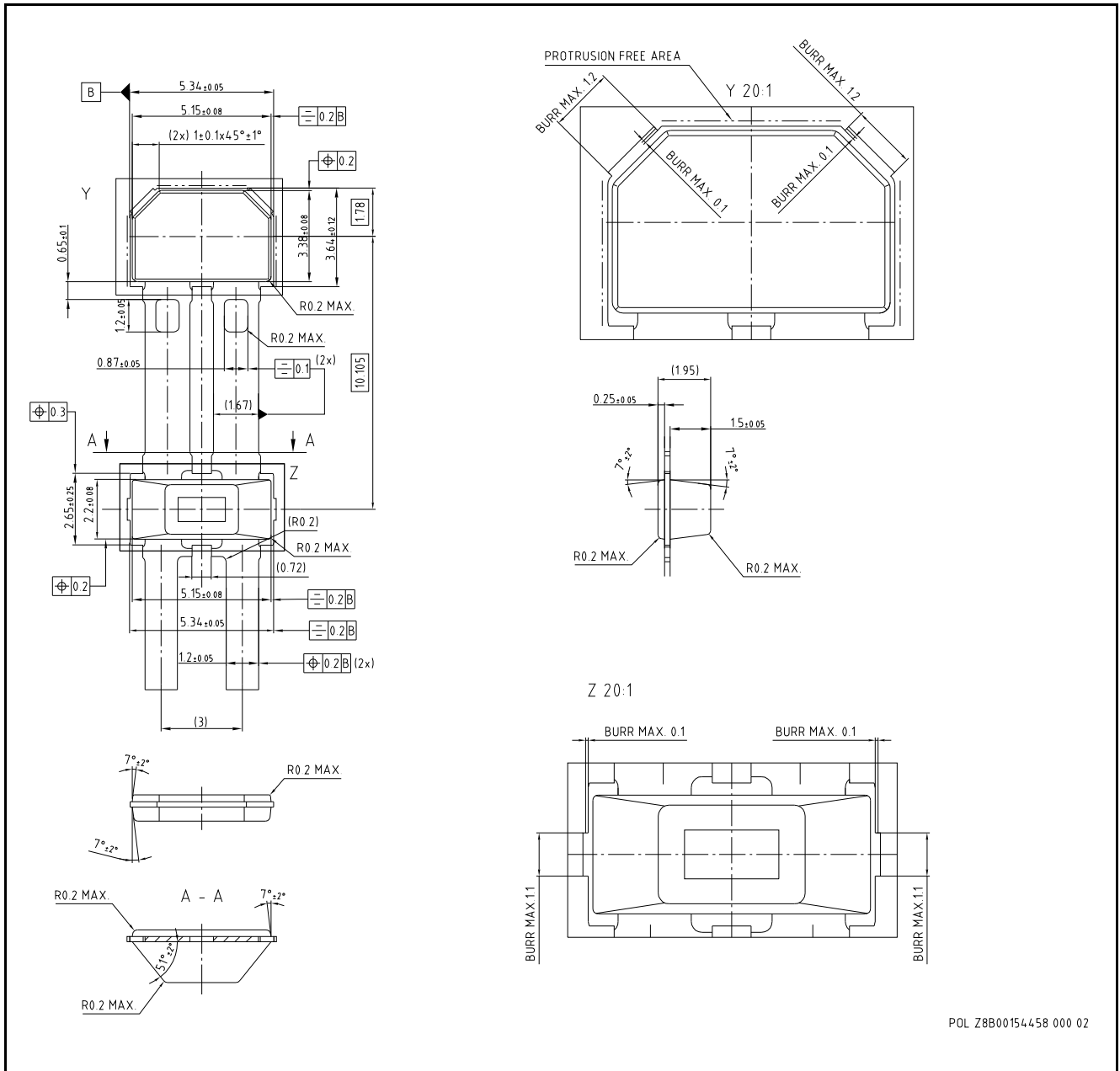
Figure 21 Package dimensions
