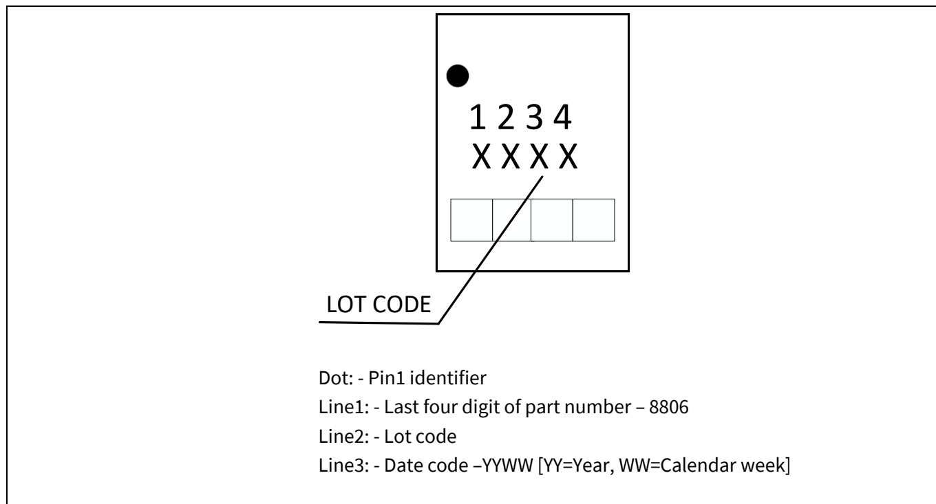
Figure 15 Package Marking
