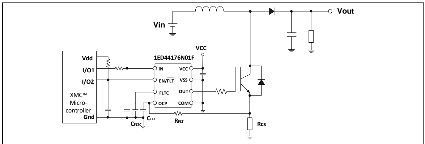
Figure 5 Application circuit example of active power factor correction (APFC) with R CS for OCP
