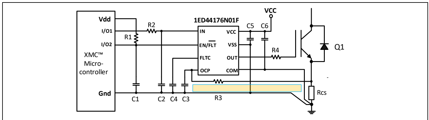
Figure 6 Recommended layout pattern for OCP & SCP function
