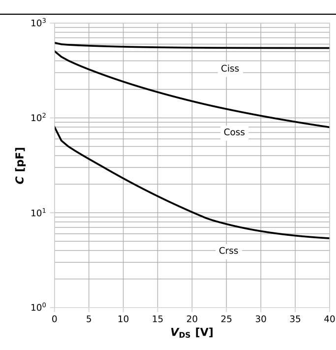
Diagram 11: Typ. capacitances (n-channel)
