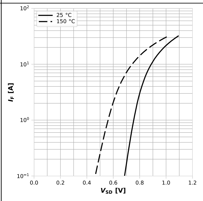
Diagram 12: Forward characteristics of reverse diode (n-ch.)
