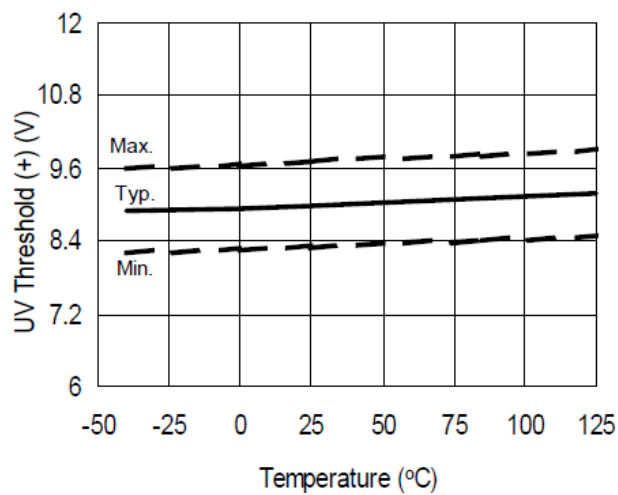
Figure 17. V_{CC} and V_{BS} Undervoltage Threshold (+) vs. Temperature
