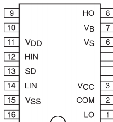
16-Lead SOIC (Wide Body)
