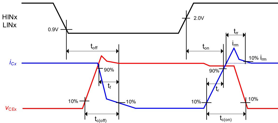
Figure 9 Switching time definition application guide
