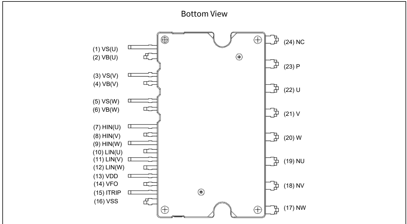
Figure 2 Pin configuration
