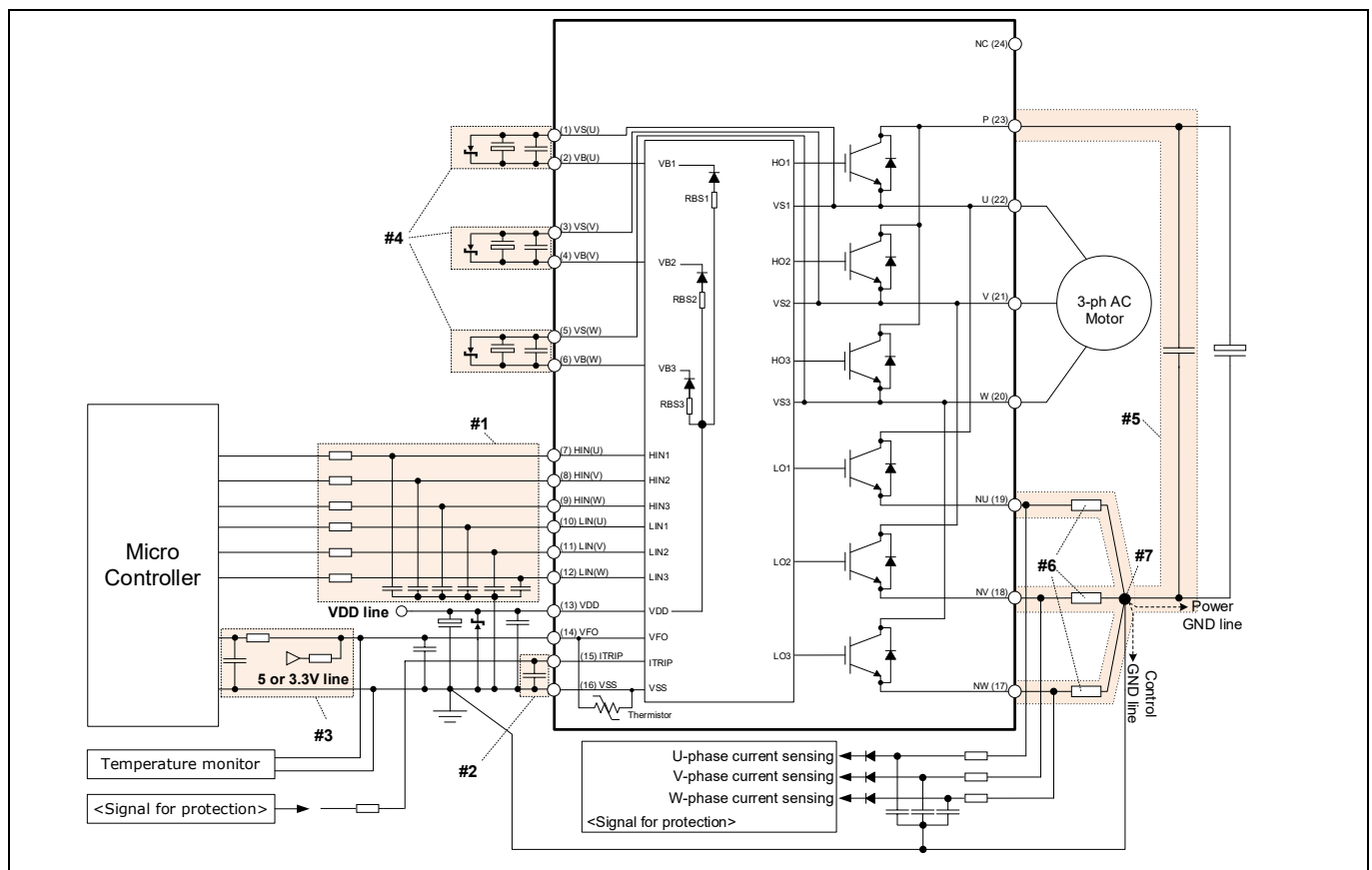
Figure 10 Typical application circuit
