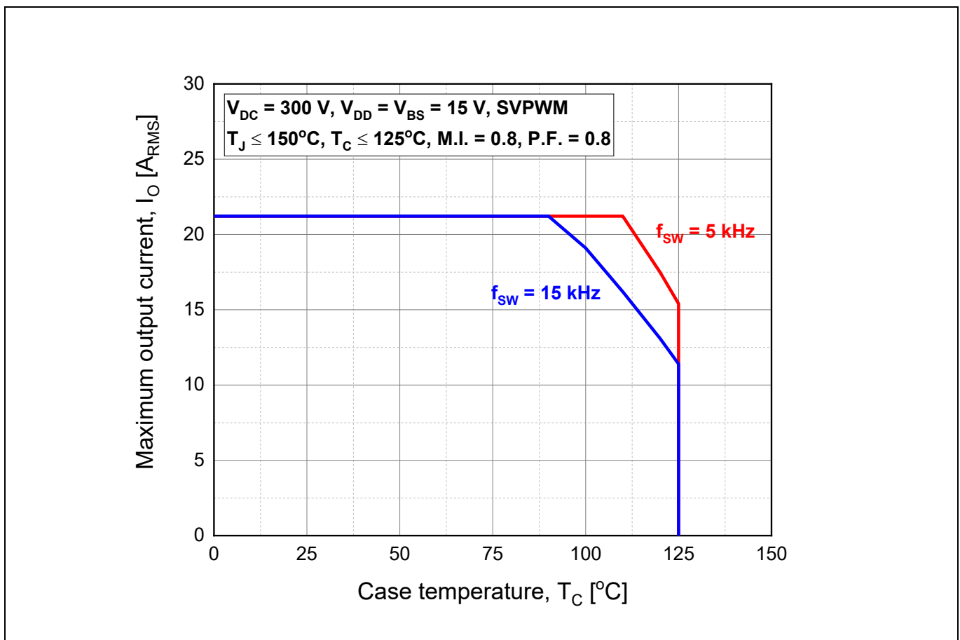
Figure 11 Maximum operating current SOA 1
