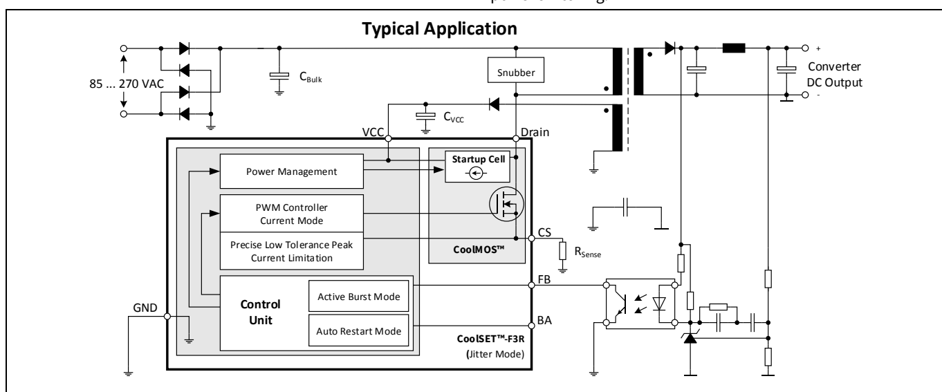
Figure 1 Typical application
