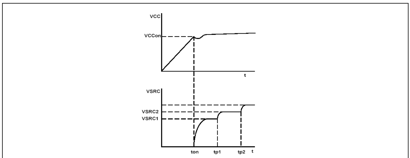
In the Startup Phase, the IC provides a Soft Start period to control the primary current by means of a duty cycle limitation. The Soft Start function is a built-in function and it is controlled by an internal counter.
