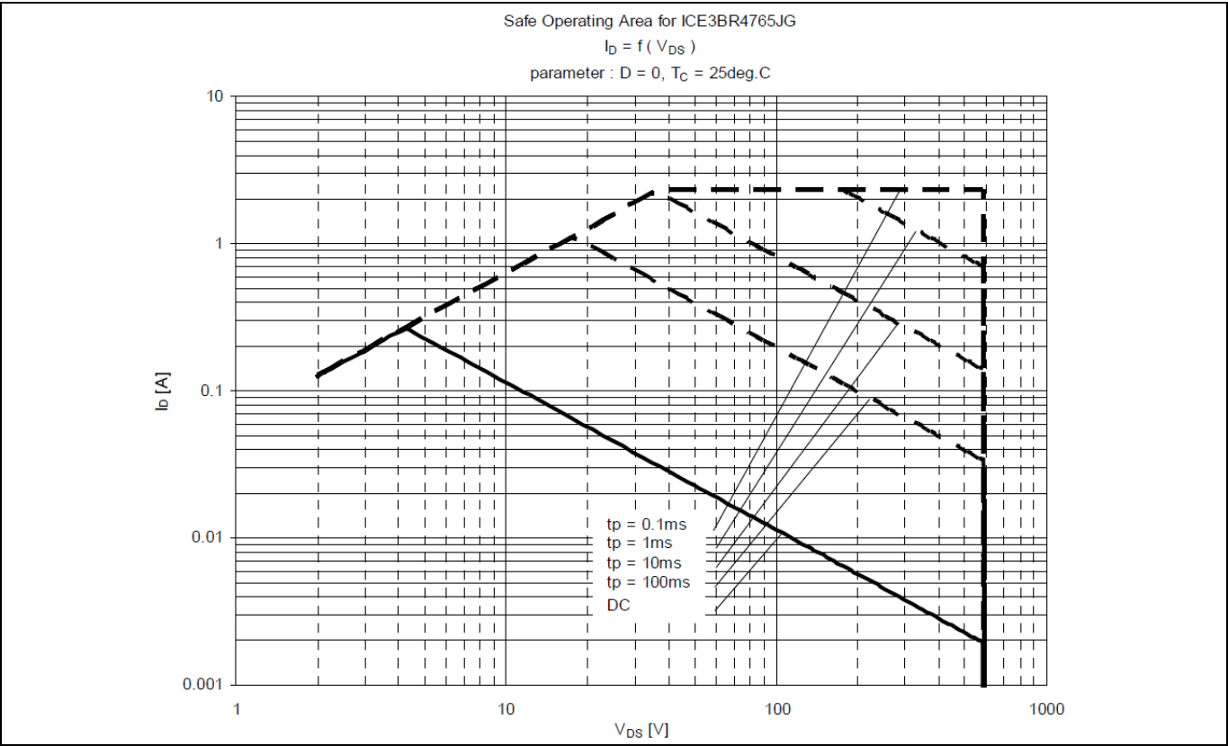
Figure 28 Safe Operating Area (SOA) curve for ICE3BR4765JG
