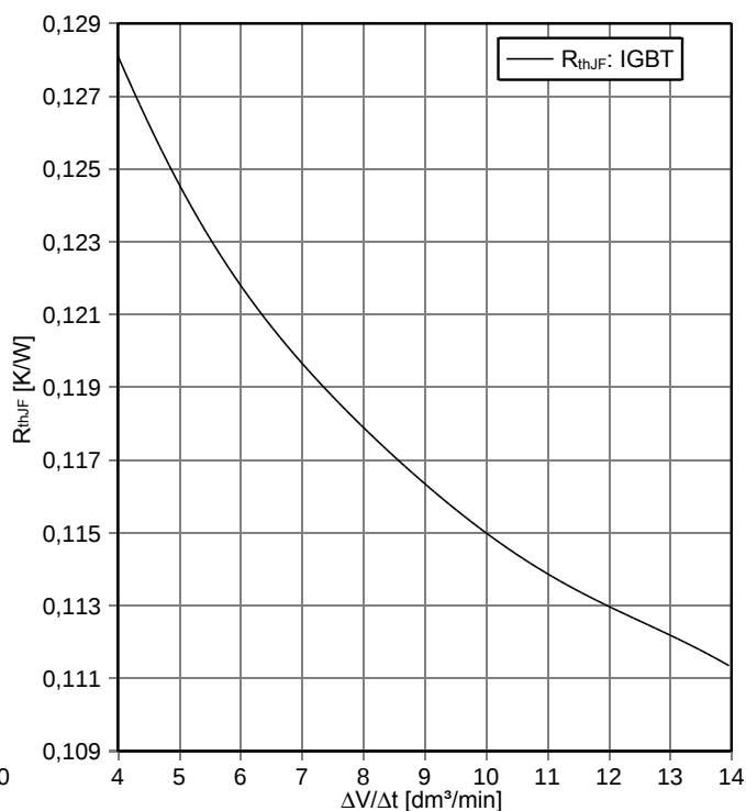
thermal impedance IGBT, Inverter
