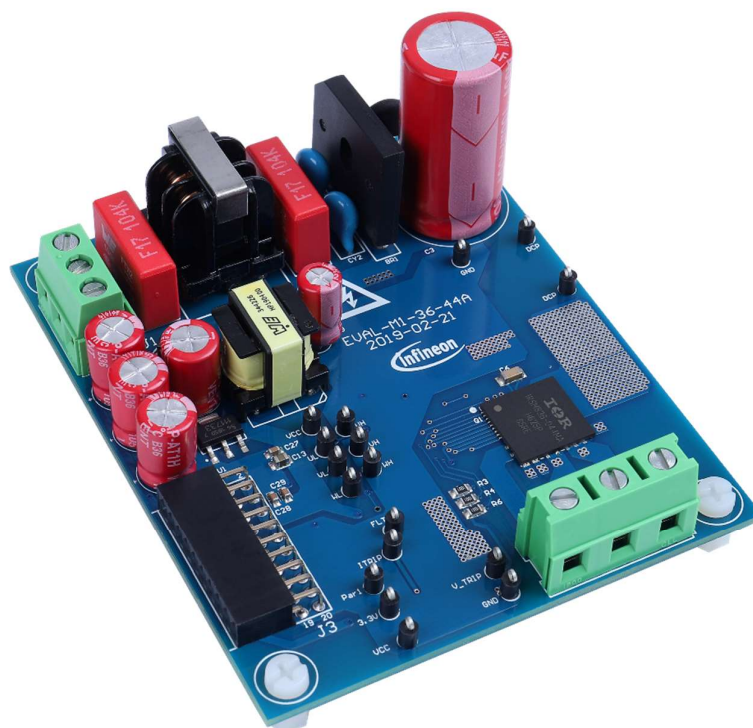
Figure 1 Evaluation-board EVAL-M1-36-44A
