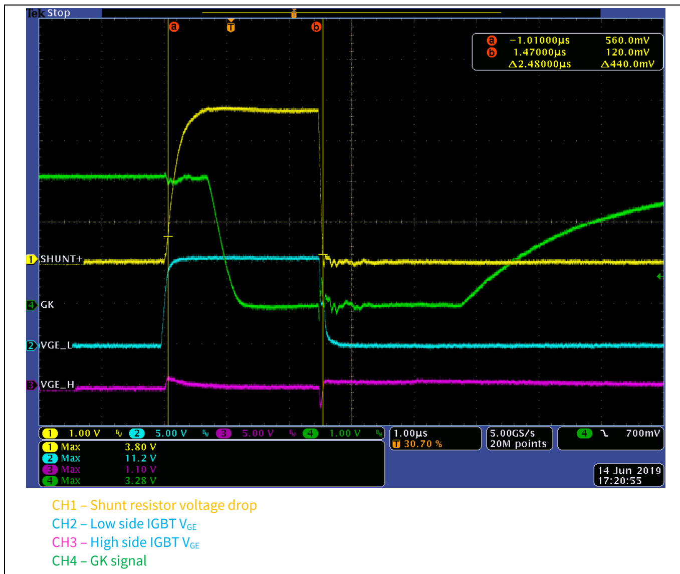
Figure 12 Test result - SCP
