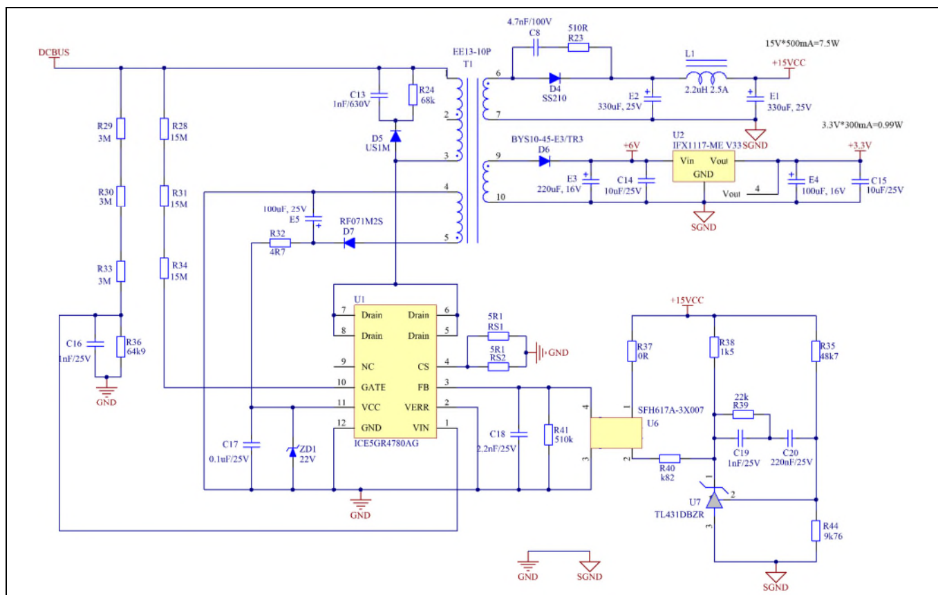
Figure 13 Auxiliary power supply circuit
