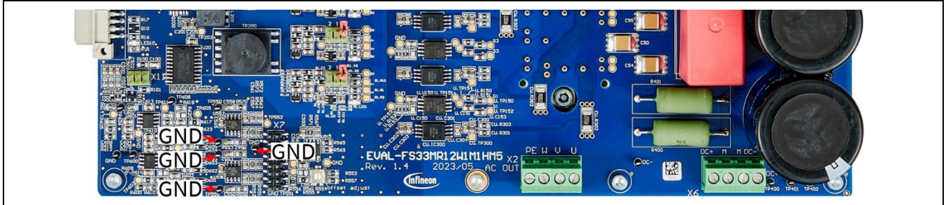
Figure 4 Relevant parts for offset adjustments
