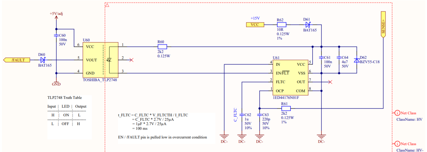
Figure 20 Short-circuit protection
