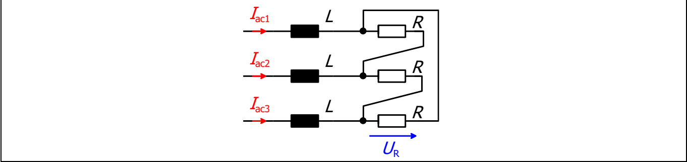
Figure 23 Test load
