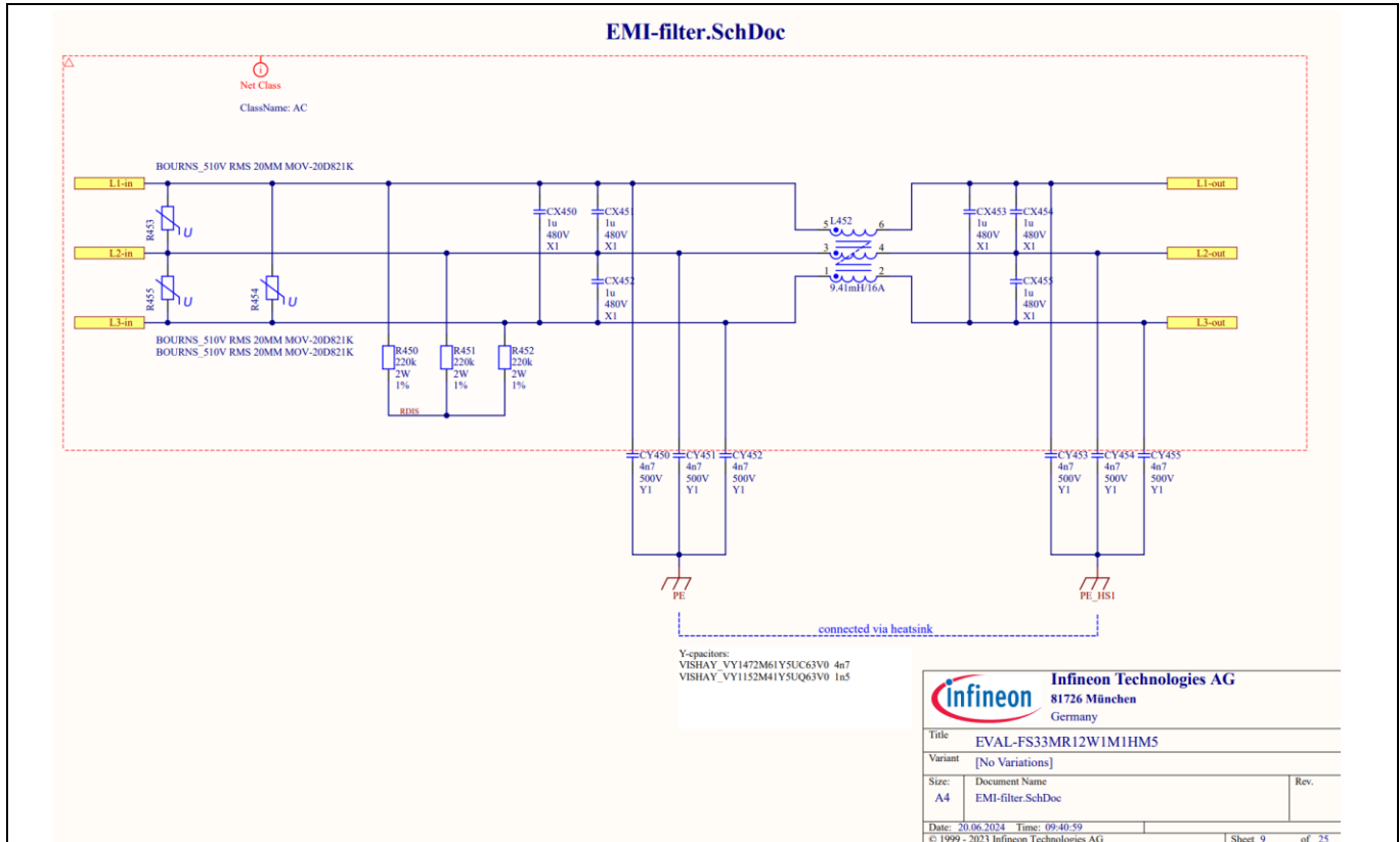
Figure 7 EMI filter
