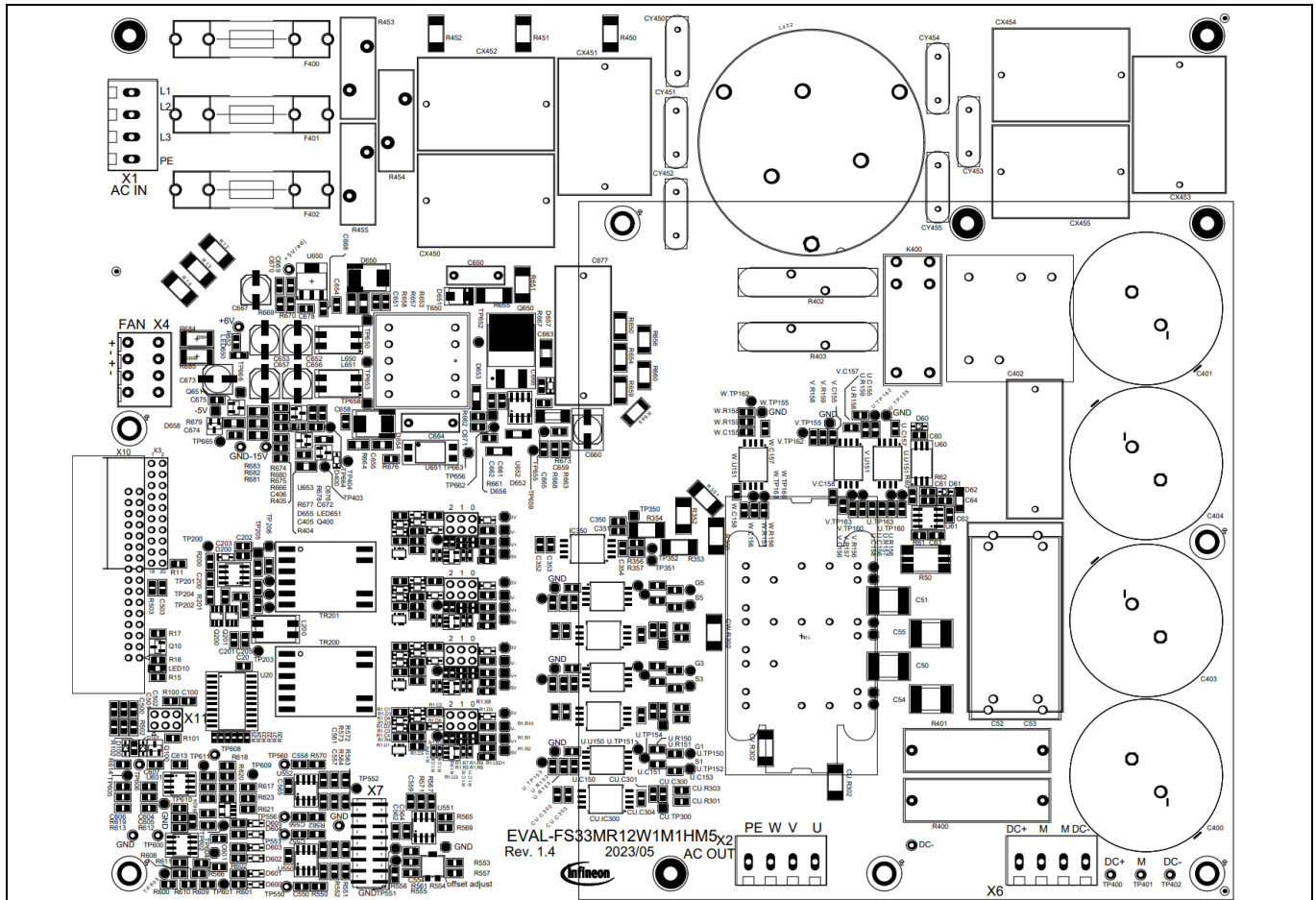
Figure 21 Top assembly print of the EVAL-FS33MR12W1M1HM5 evaluation board
