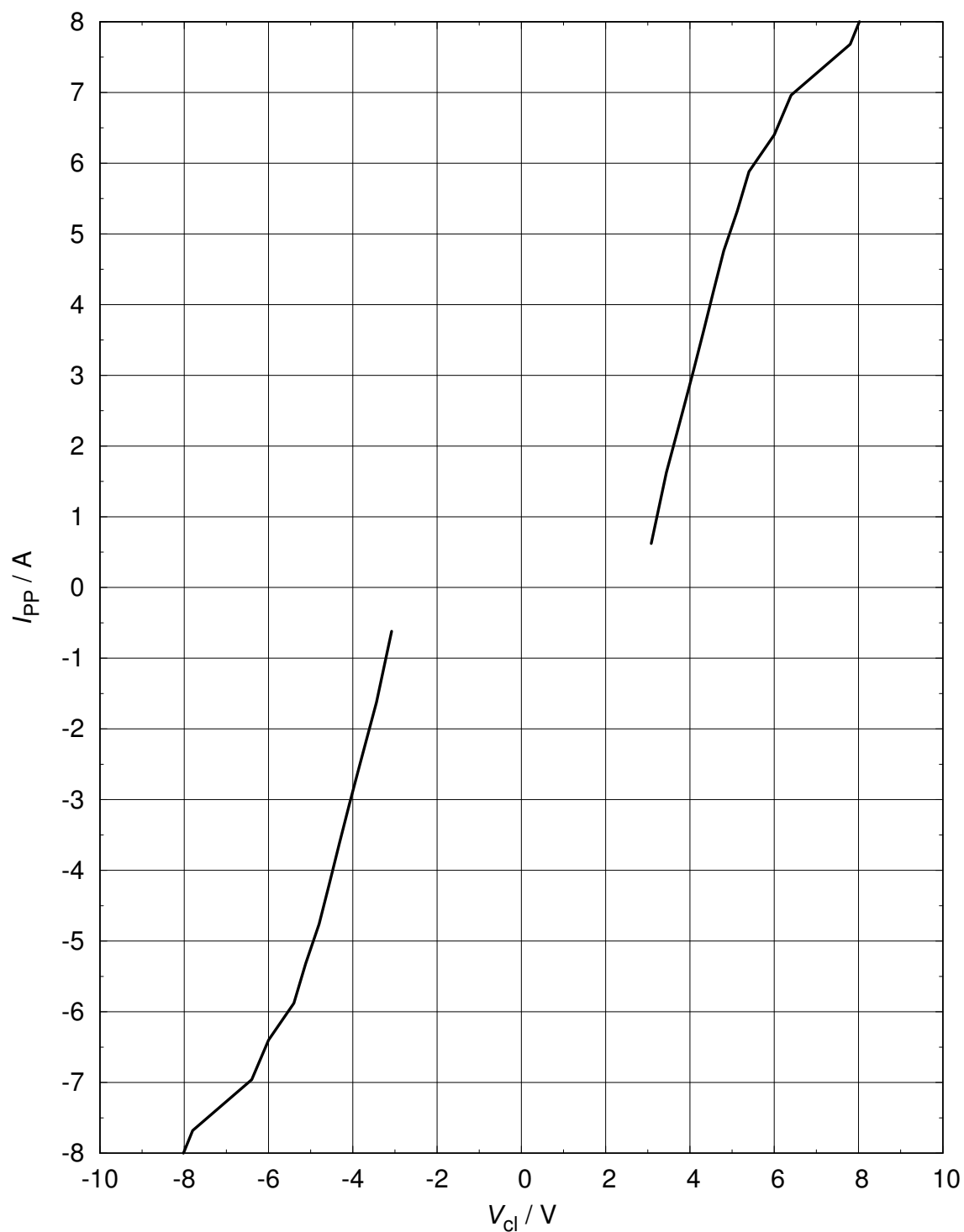
Figure 12 Clamping voltage (Surge): I_{PP} = f(V_{CL}) , based on IEC61000-4-5
