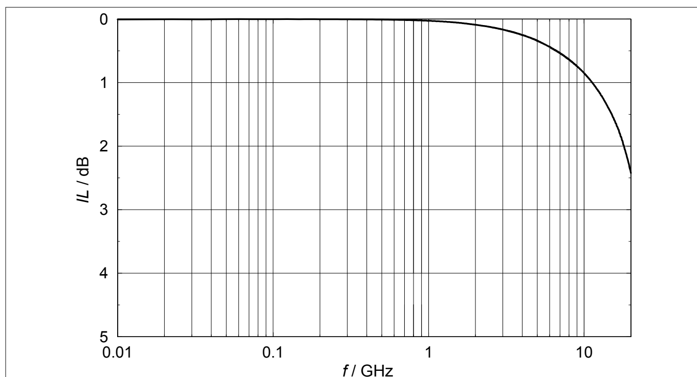
Figure 6 Insertion loss IL = f(f) , measured in a 50 \Omega system
