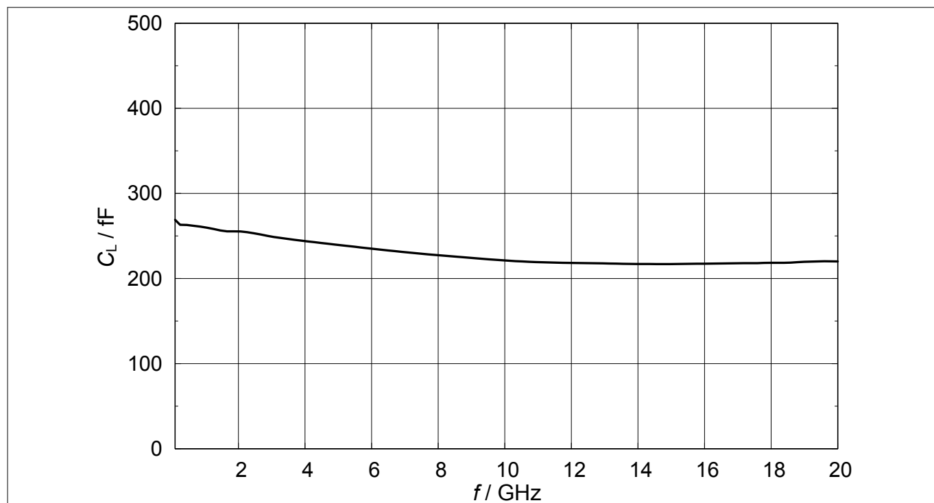
Figure 5 Line capacitance: C_L = f(f) = 1 \text{ MHz}
